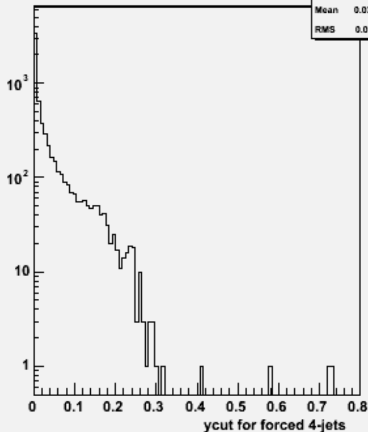
Ycut for 4-jets :w100816 e2e2n2e2e1n1_o
