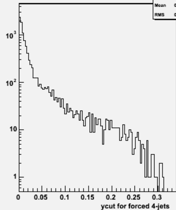
Ycut for 4-jets :w100813 e2e2n1e1sc_o
