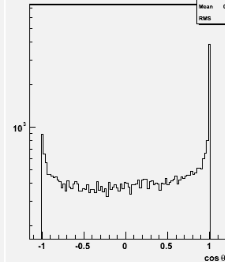
Jet cos \theta (All jets)w100813 e2e2n1e1sc_o
