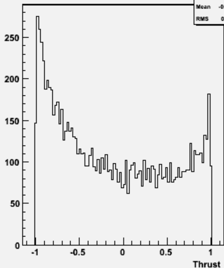
cos \Theta (thrust) w100813 e2e2n1e1sc_o
