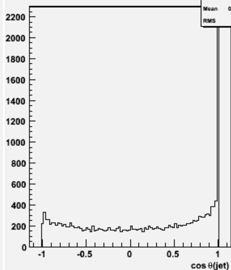
cos \theta for 2-jets :w100813 e2e2n1e1sc_o
