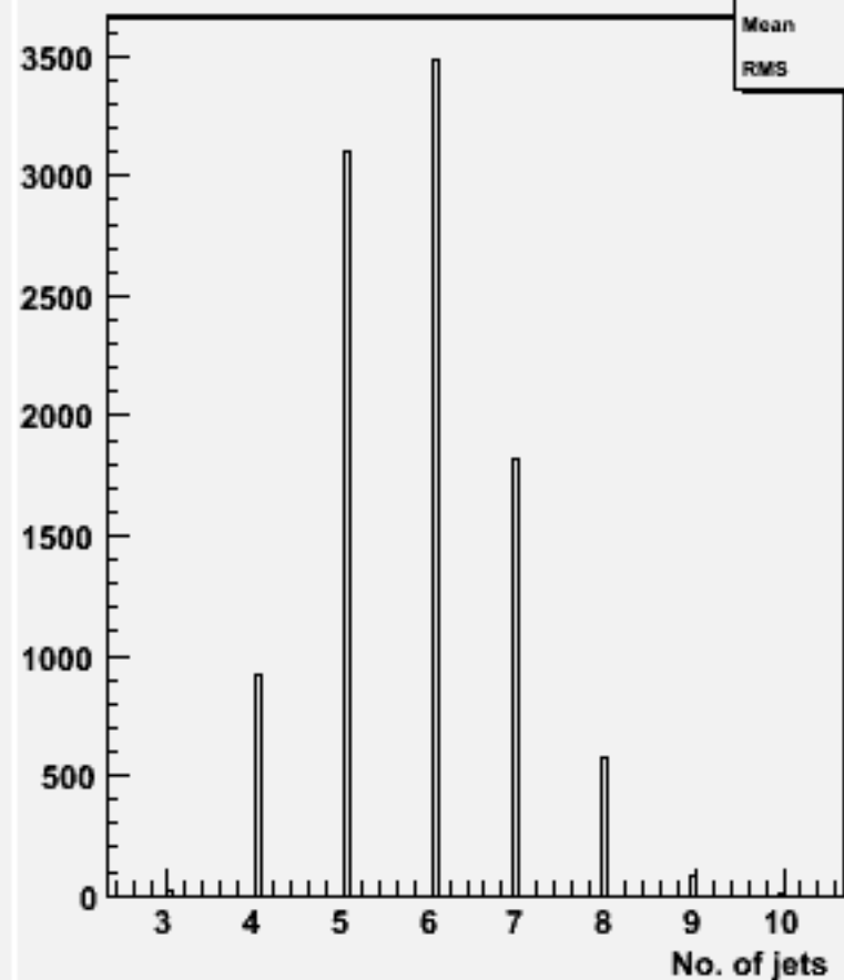
No. jets (ycut=0.001) : w100813 e2e2n1e1sc_o
