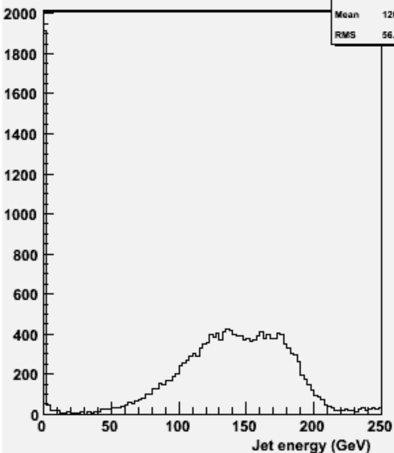
energy for 2-jets :w100813 e2e2n1e1sc_o
