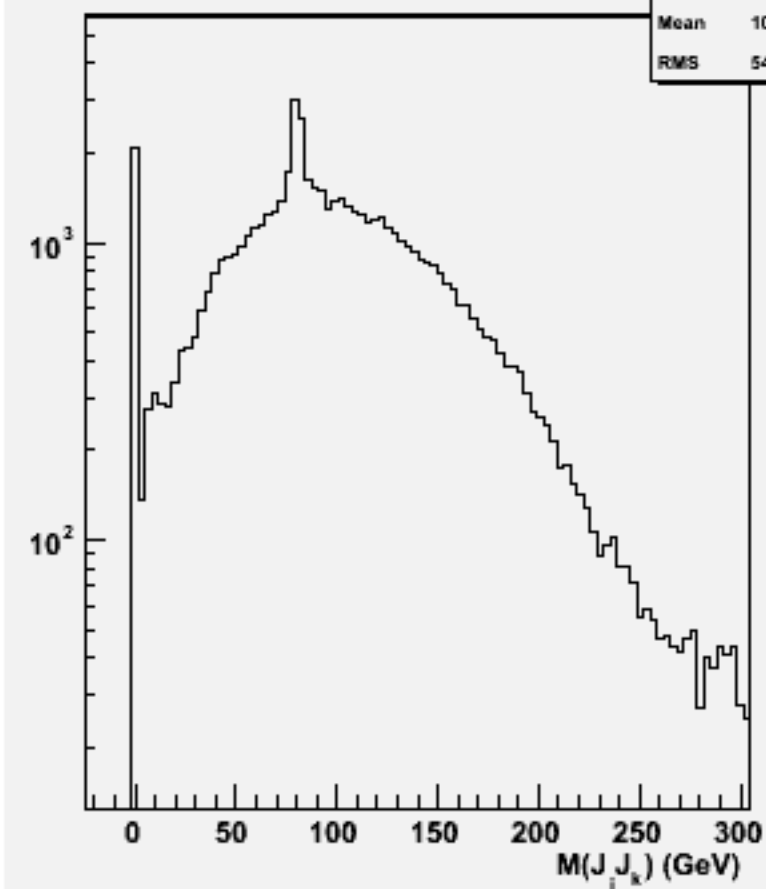
2jets mass(All comb)w100813 e2e2n1e1sc_o
