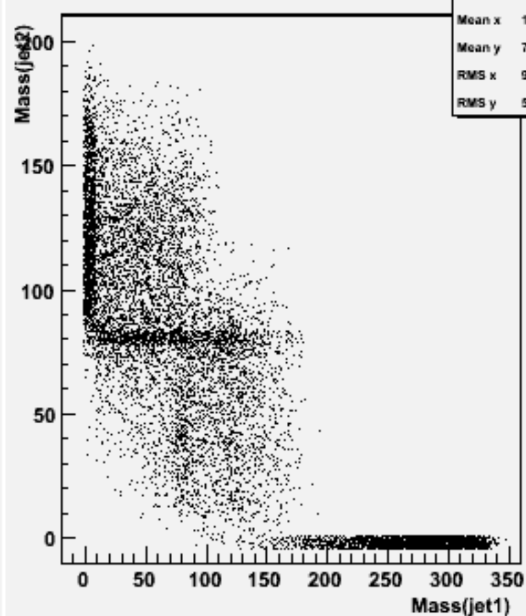
Jet mass for forced 2-jets : w100813 e2e2n1e1sc_o
