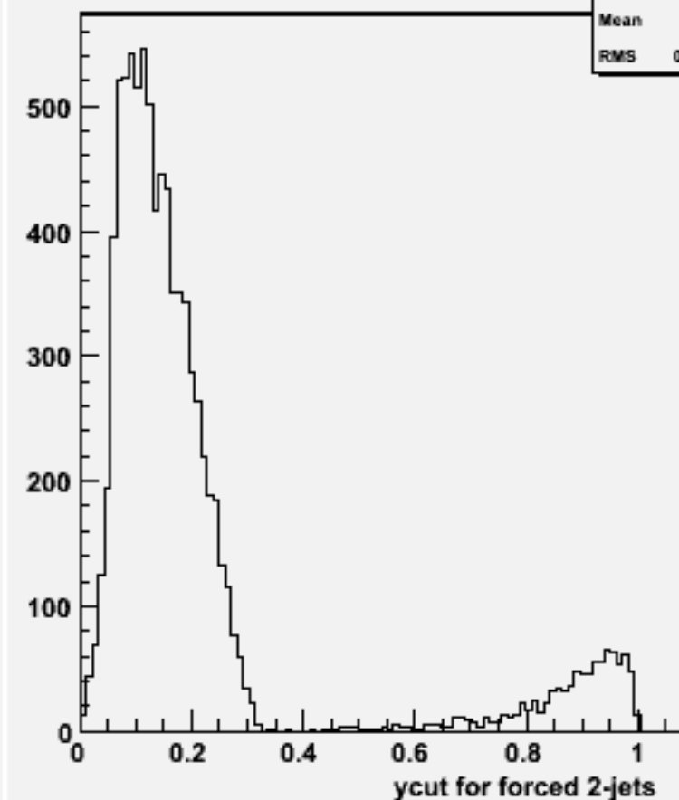
Ycut for 2-jets :w100813 e2e2n1e1sc_o
