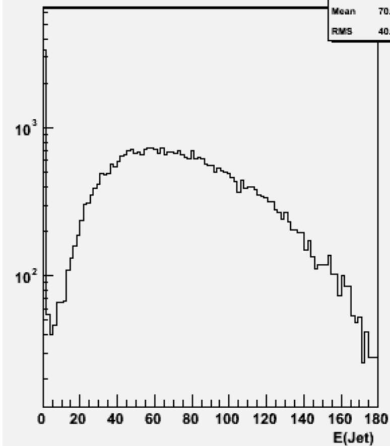
Jet energies(All jets)w100812 e2e2n1e1sc_o
