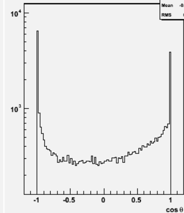
Jet cos \theta (All jets)w100812 e2e2n1e1sc_o
