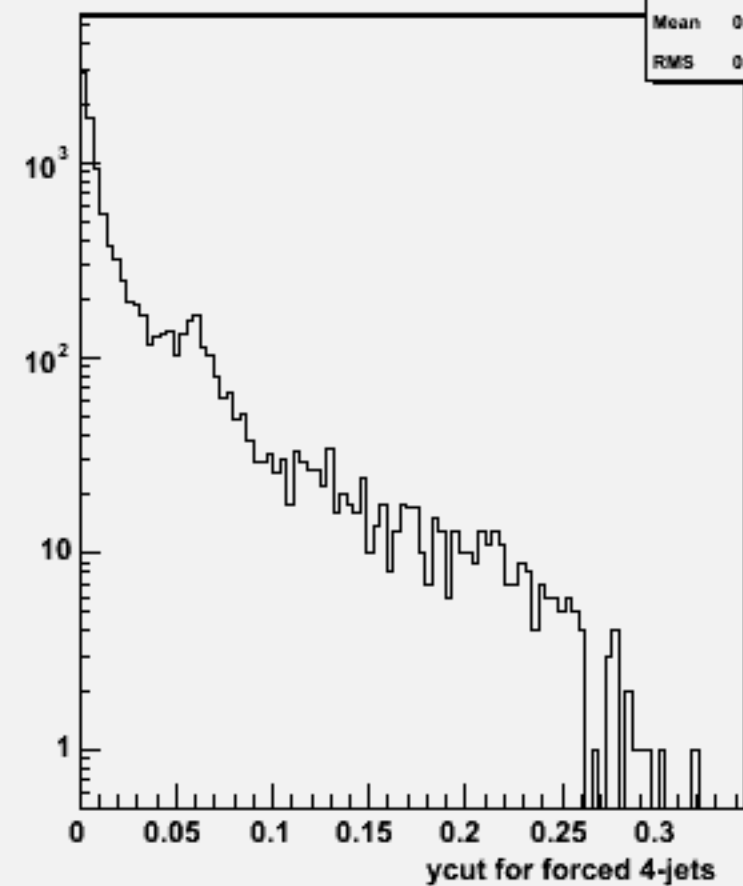
Ycut for 4-jets :w100812 e2e2n1e1sc_o
