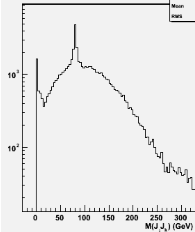
2jets mass(All comb)w100812 e2e2n1e1sc_o
