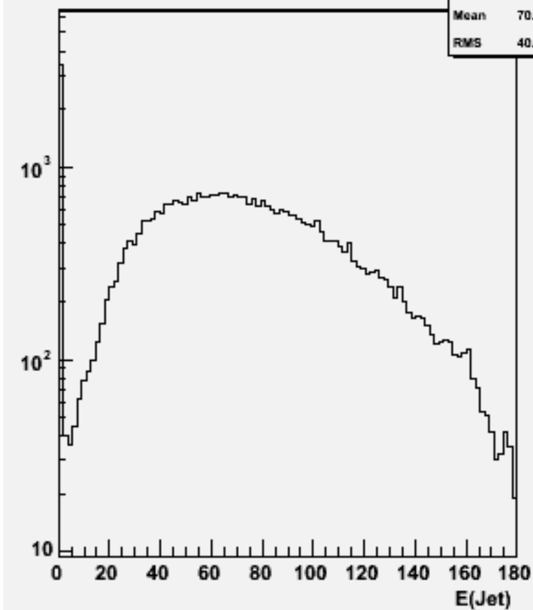
Jet energies(All jets)w100811 e2e2n1e1sc_o
