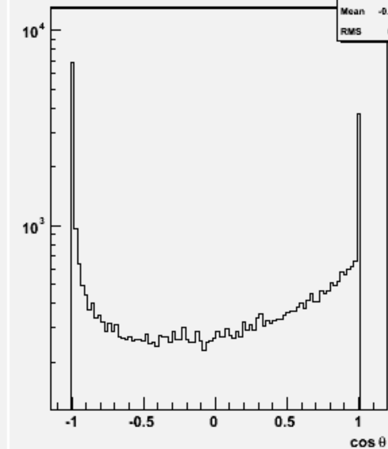
Jet cos \theta (All jets)w100811 e2e2n1e1sc_o
