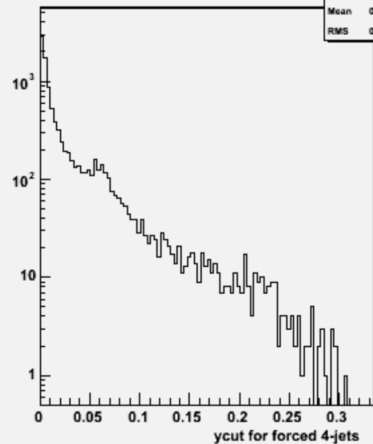
Ycut for 4-jets :w100811 e2e2n1e1sc_o
