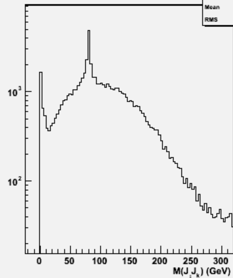
2jets mass(All comb)w100811 e2e2n1e1sc_o
