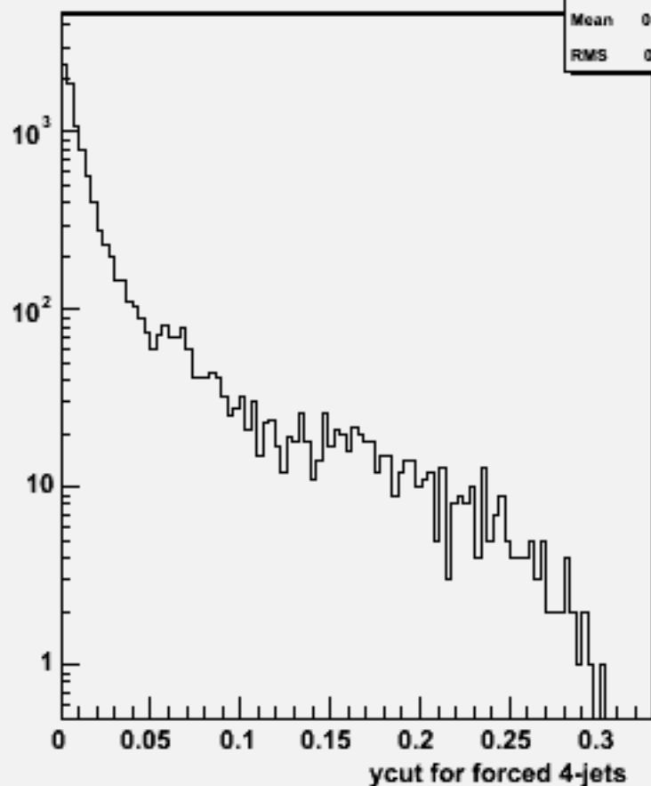
Ycut for 4-jets :w100809 e2e2n1e1du_o
