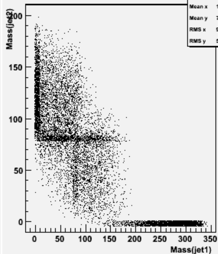
Jet mass for forced 2-jets : w100809 e2e2n1e1du_o
