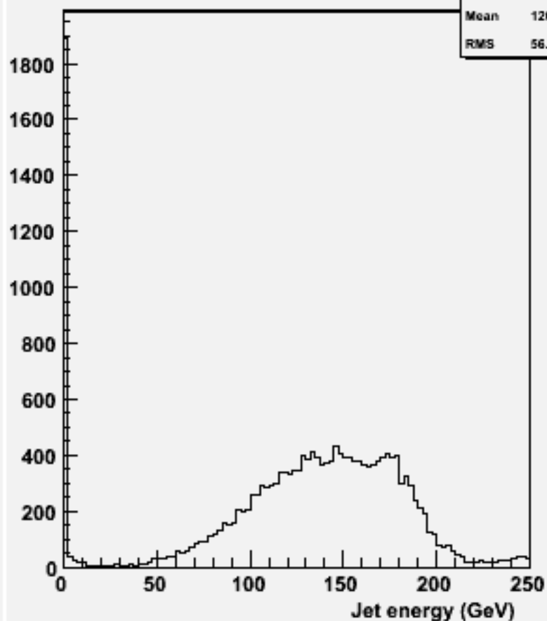
energy for 2-jets :w100809 e2e2n1e1du_o
