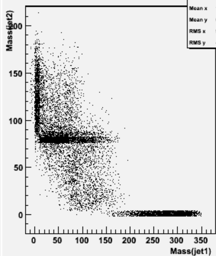
Jet mass for forced 2-jets : w100807 e2e2n1e1du_o
