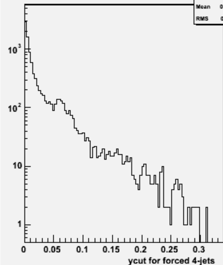
Ycut for 4-jets :w100807 e2e2n1e1du_o
