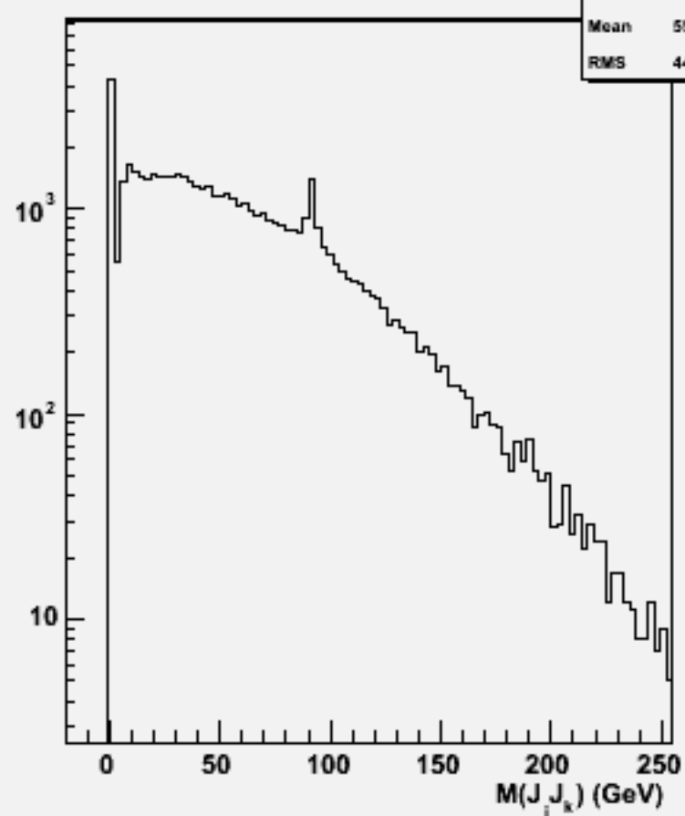
2jets mass(All comb)w100805 e2e2n1e1e3n3_o
