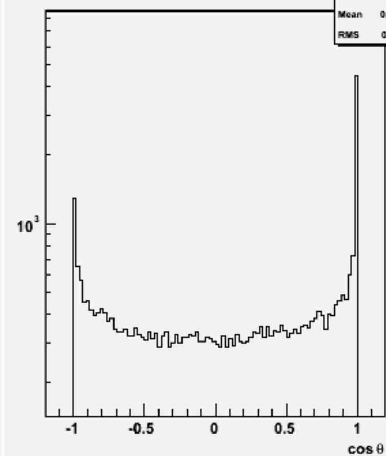
Jet cos \theta (All jets)w100805 e2e2n1e1e3n3_o
