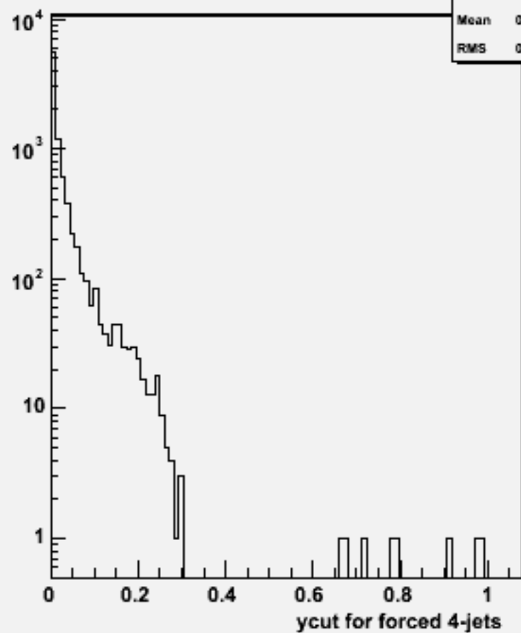
Ycut for 4-jets :w100805 e2e2n1e1e3n3_o
