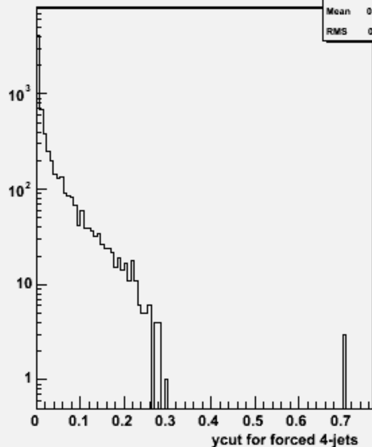
Ycut for 4-jets :w100804 e2e2n1e1e3n3_o
