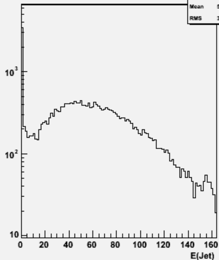
Jet energies(All jets)w100798 e2e2n1e1e1n1_o
