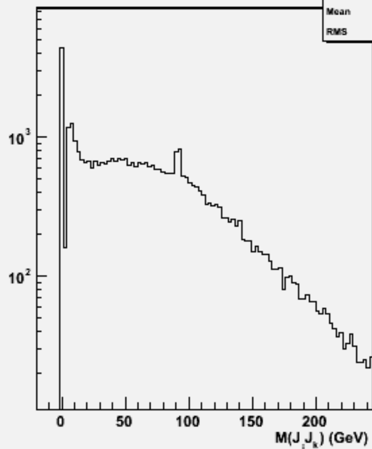
2jets mass(All comb)w100798 e2e2n1e1e1n1_o
