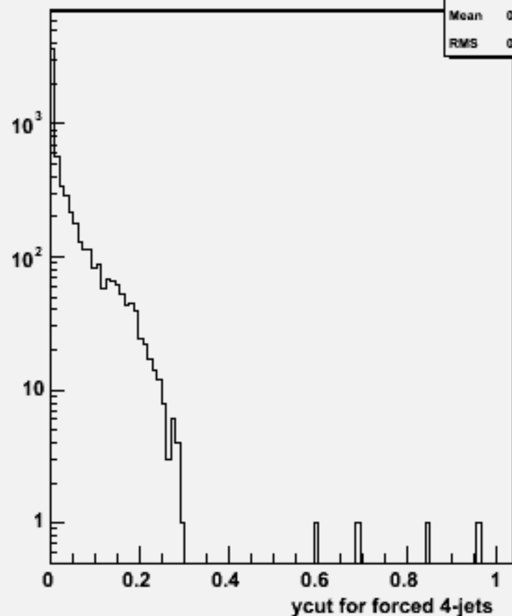
Ycut for 4-jets :w100798 e2e2n1e1e1n1_o
