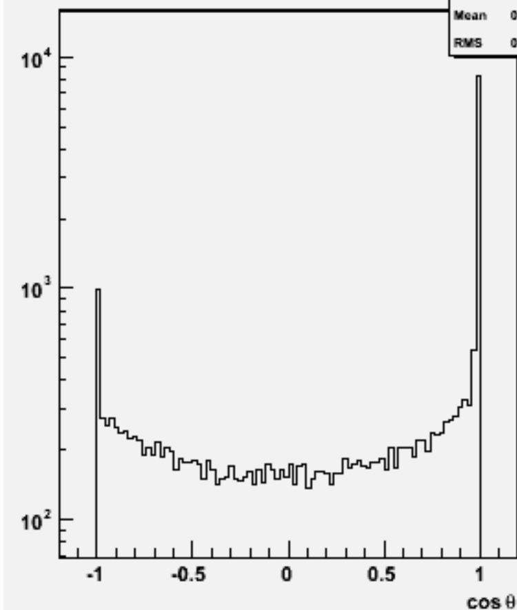
Jet cos \theta (All jets)w100798 e2e2n1e1e1n1_o
