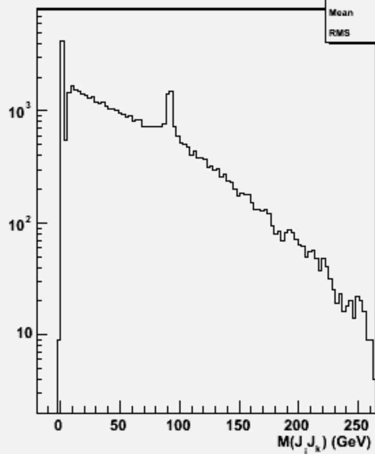
2jets mass(All comb)w100797 e2e2n1e1e1n1_o
