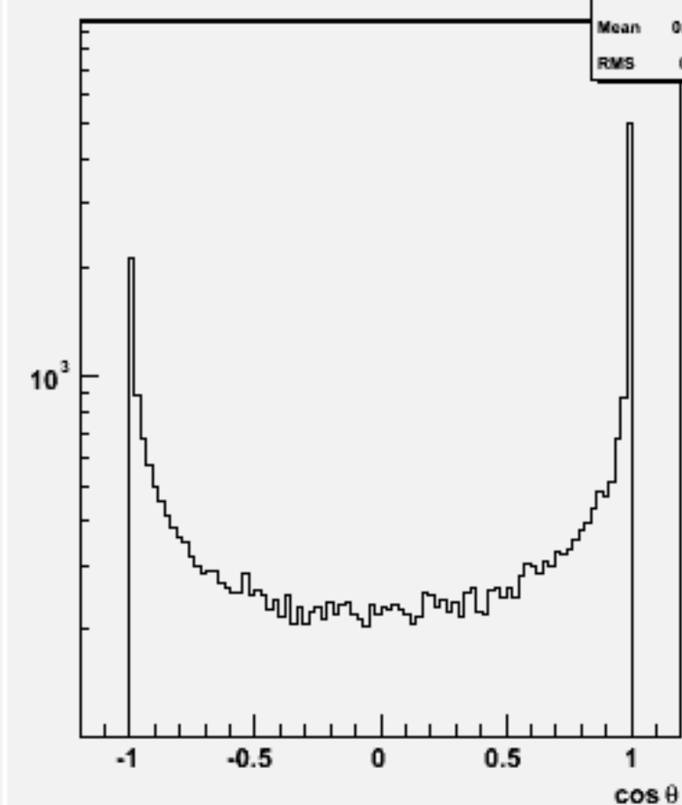
Jet cos \theta (All jets)w100797 e2e2n1e1e1n1_o
