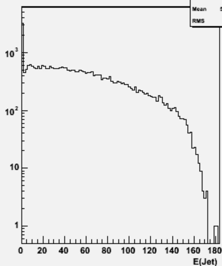
Jet energies(All jets)w100797 e2e2n1e1e1n1_o
