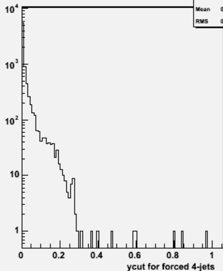
Ycut for 4-jets :w100797 e2e2n1e1e1n1_o
