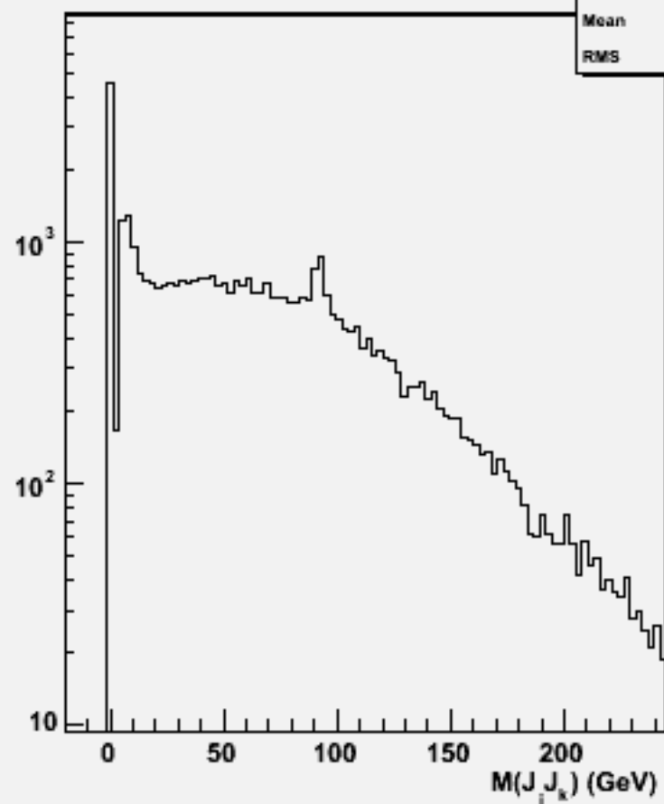
2jets mass(All comb)w100796 e2e2n1e1e1n1_o
