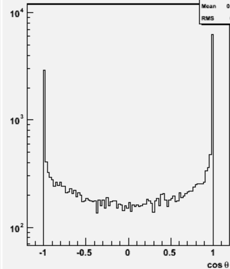
Jet cos \theta (All jets)w100796 e2e2n1e1e1n1_o
