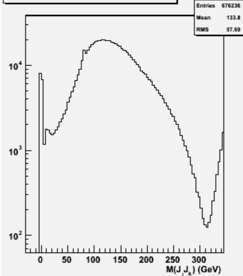
2jets mass(All comb)w100794 e1e1cssc_o
