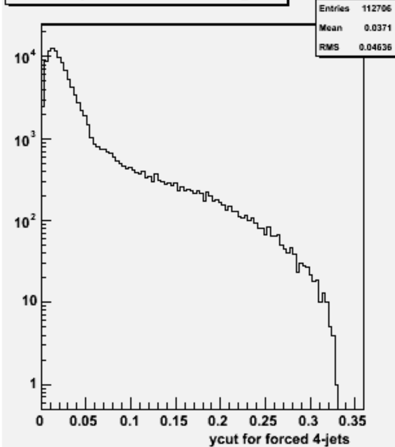
Ycut for 4-jets :w100794 e1e1cssc_o
