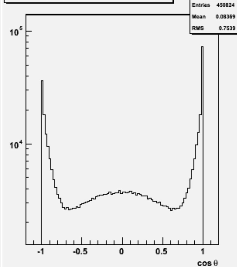
Jet cos \theta (All jets)w100794 e1e1cssc_o
