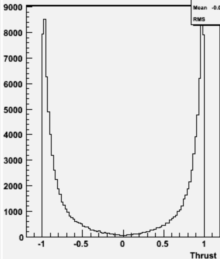
cos \Theta (thrust) w100793 e1e1cssc_o
