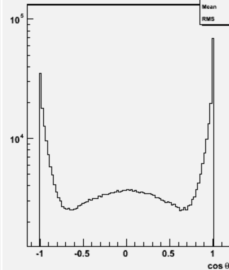
Jet cosθ (All jets)w100793 e1e1cssc_o
