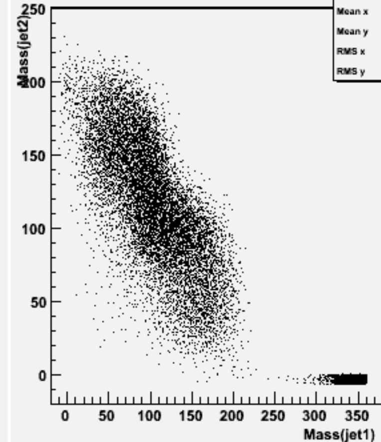
Jet mass for forced 2-jets : w100793 e1e1cssc_o
