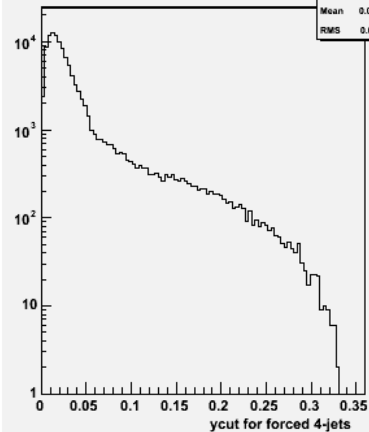
Ycut for 4-jets :w100793 e1e1cssc_o
