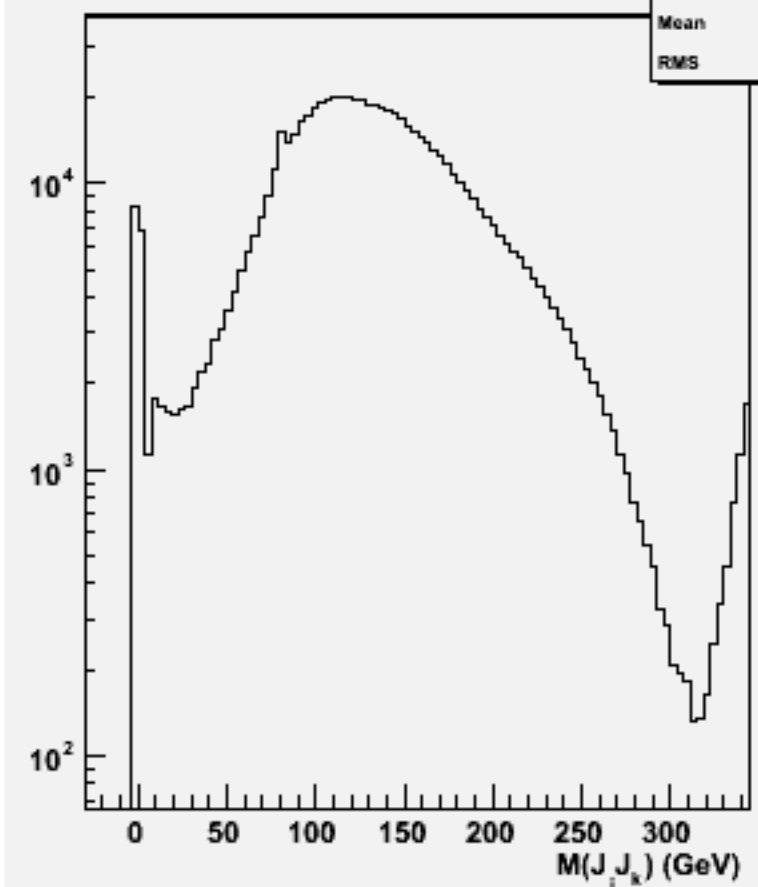
2jets mass(All comb)w100793 e1e1cssc_o
