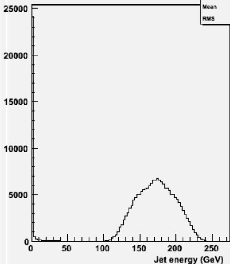
energy for 2-jets :w100793 e1e1cssc_o
