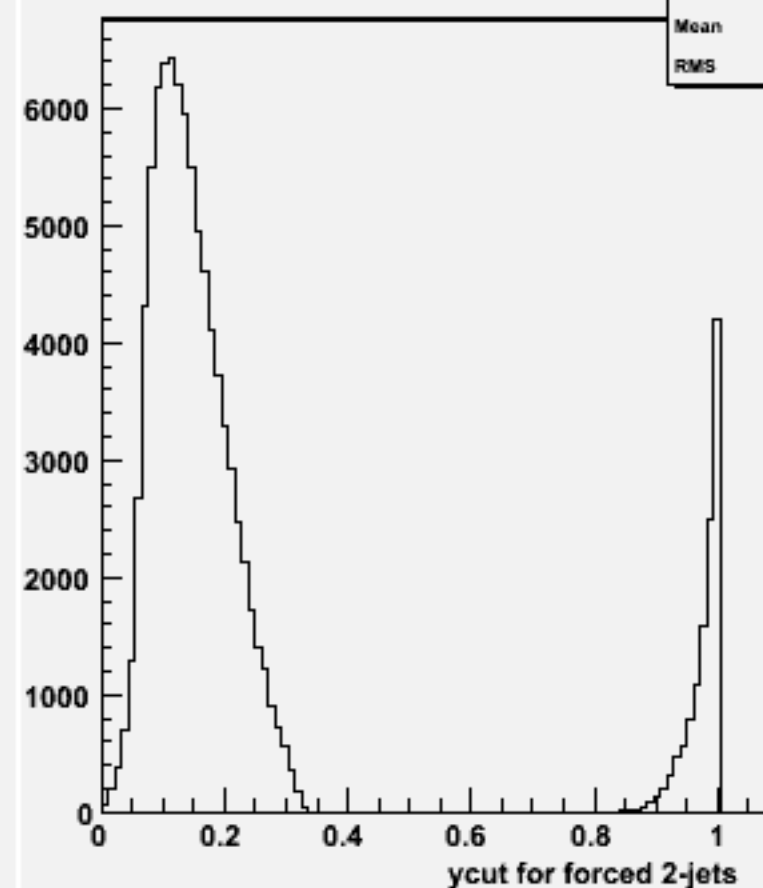
Ycut for 2-jets :w100793 e1e1cssc_o
