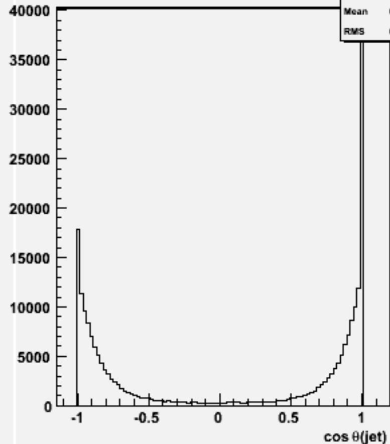
cos \theta for 2-jets :w100793 e1e1cssc_o
