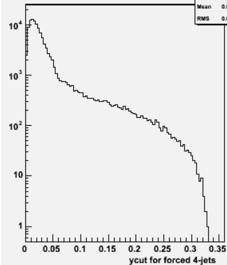
Ycut for 4-jets :w100790 e1e1csdu_o
