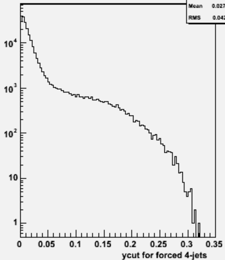
Ycut for 4-jets :w100785 e1e1cse3n3_o
