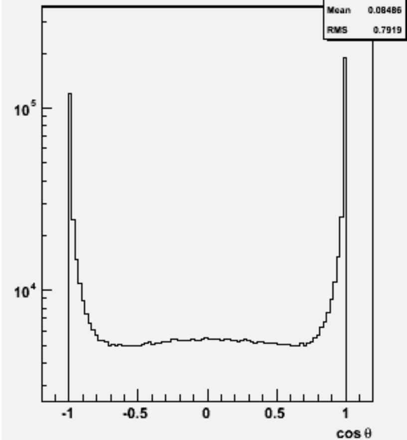
Jet cos \theta (All jets)w100785 e1e1cse3n3_o
