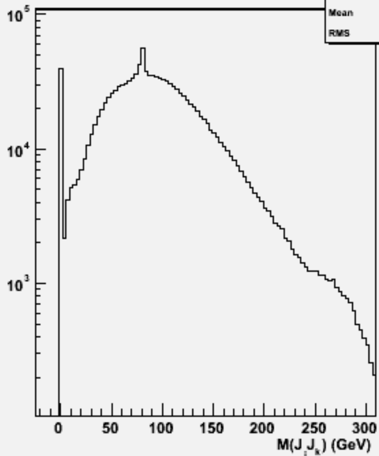
2jets mass(All comb)w100785 e1e1cse3n3_o
