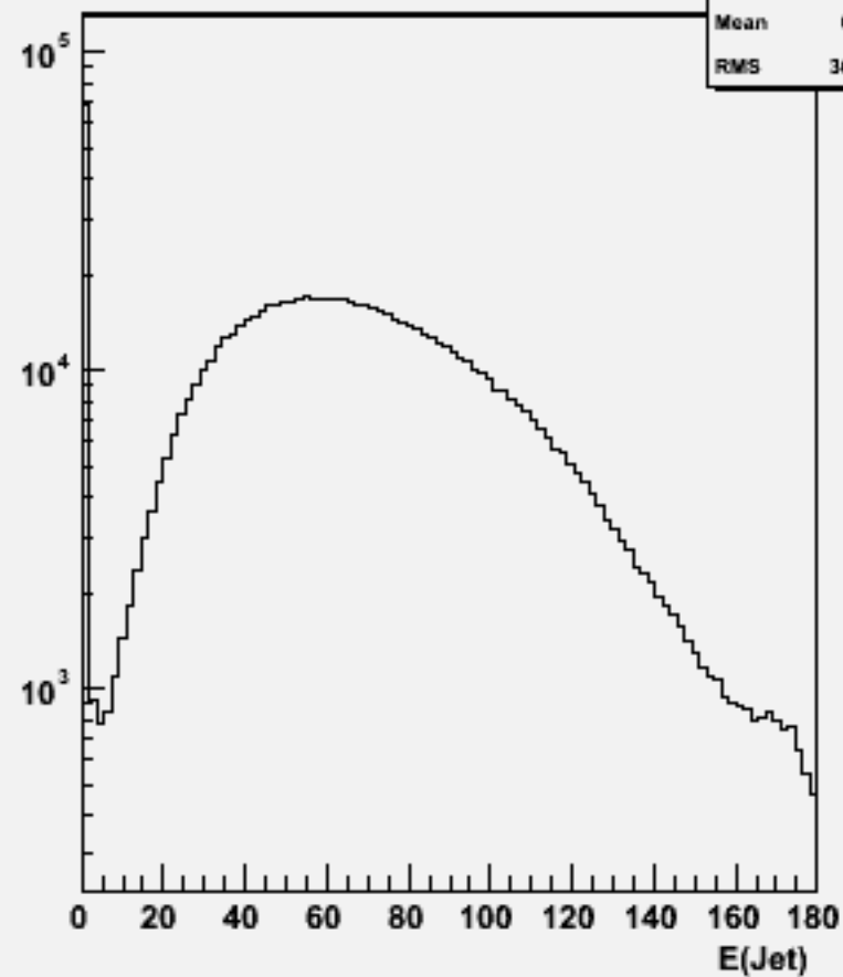
Jet energies(All jets)w100785 e1e1cse3n3_o
