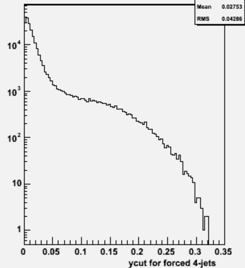
Ycut for 4-jets :w100783 e1e1cse3n3_o
