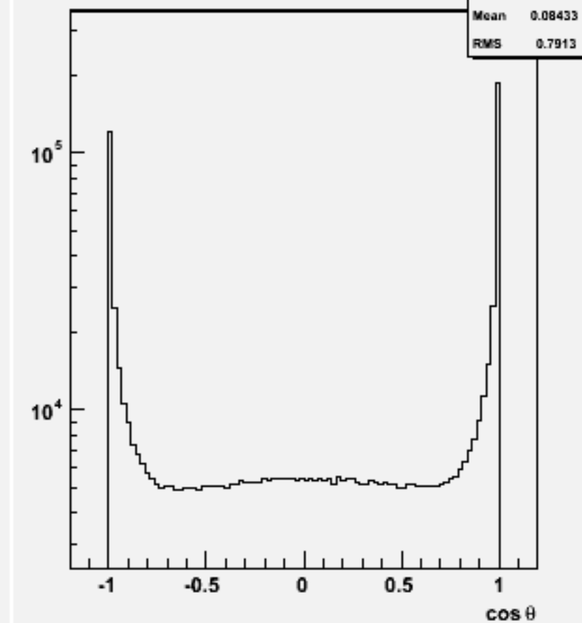
Jet cos \theta (All jets)w100783 e1e1cse3n3_o
