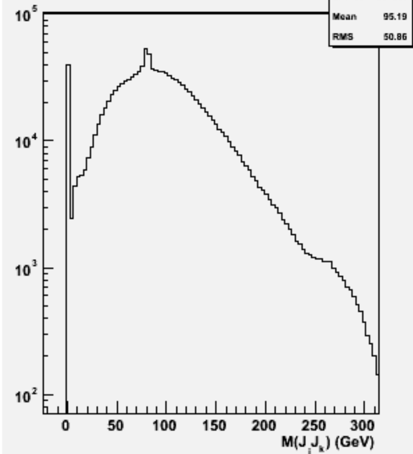
2jets mass(All comb)w100783 e1e1cse3n3_o
