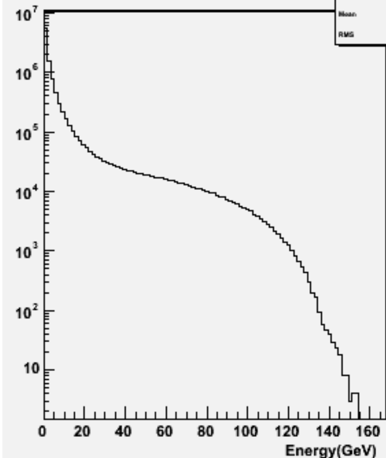
Particle Energy : w100783 e1e1cse3n3_o
