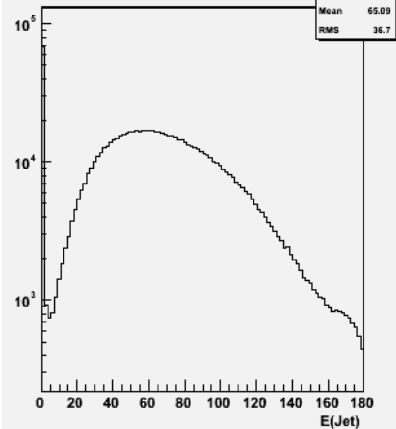
Jet energies(All jets)w100783 e1e1cse3n3_o
