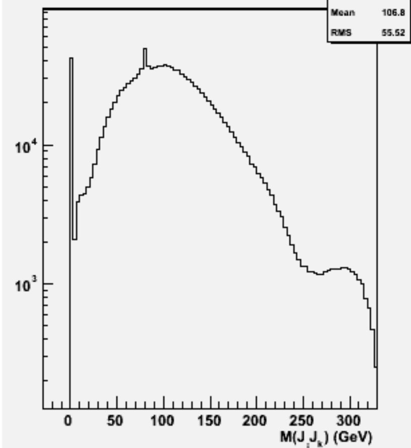
2jets mass(All comb)w100782 e1e1cse2n2_o
