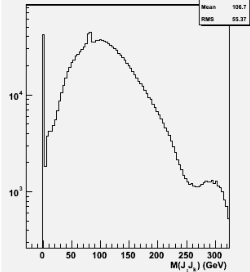
2jets mass(All comb)w100778 e1e1cse1n1_o
