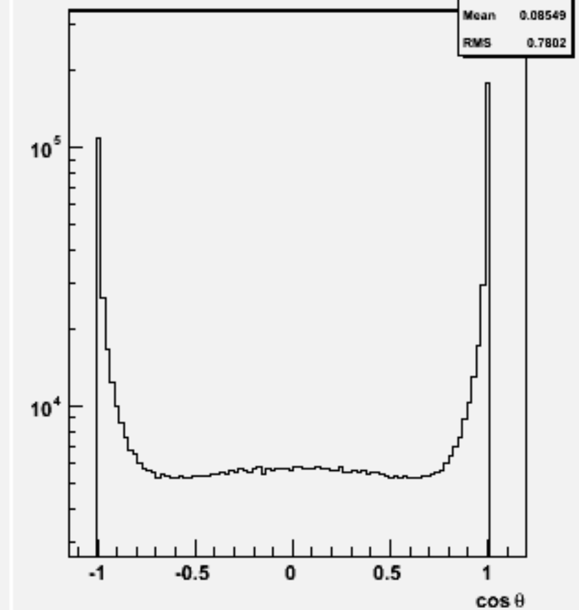
Jet cos \theta (All jets)w100778 e1e1cse1n1_o
