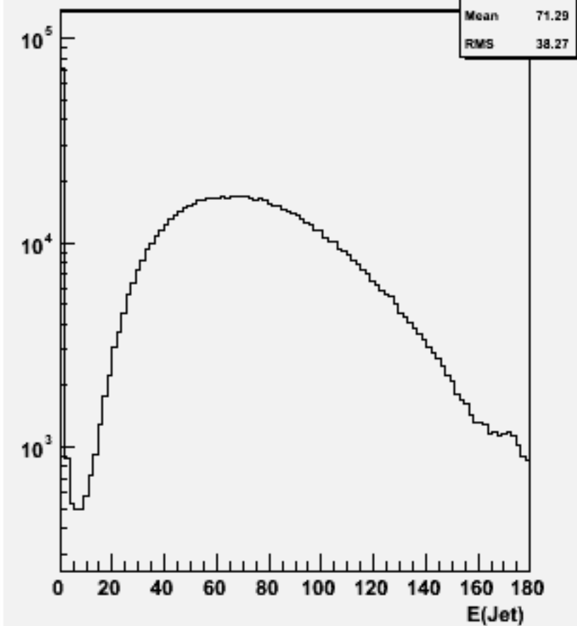
Jet energies(All jets)w100778 e1e1cse1n1_o
