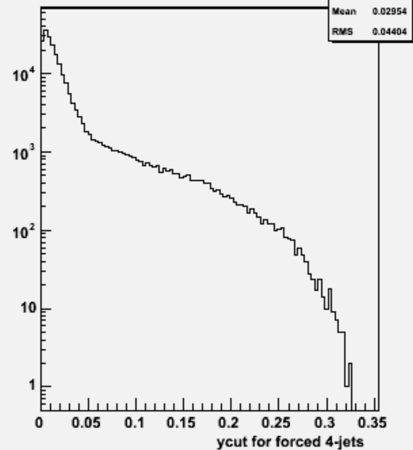
Ycut for 4-jets :w100778 e1e1cse1n1_o
