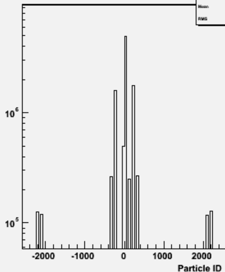
Particle ID : w100776 e1e1cse1n1_o
