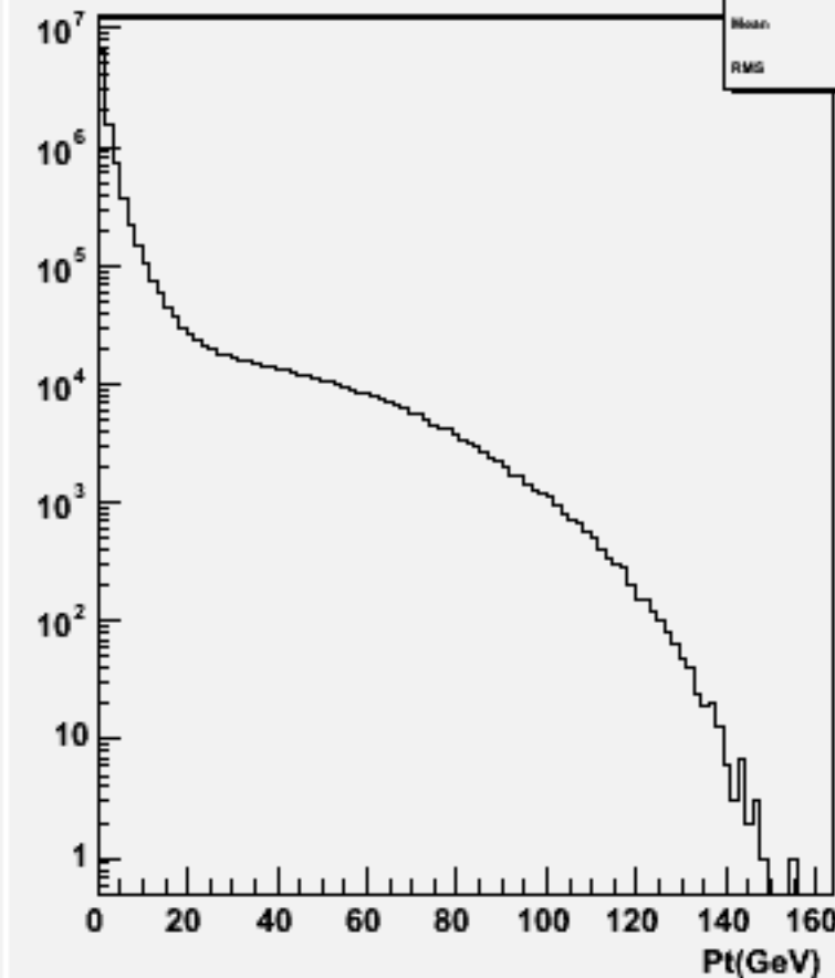
Particle Pt : w100776 e1e1cse1n1_o
