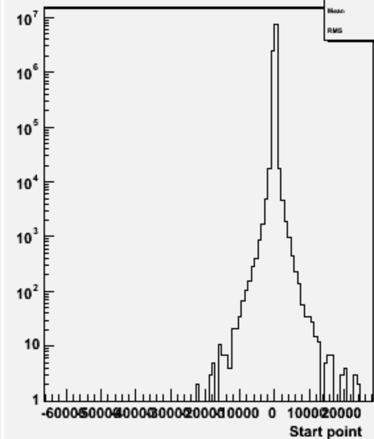
Start point Z : w100776 e1e1cse1n1_o
