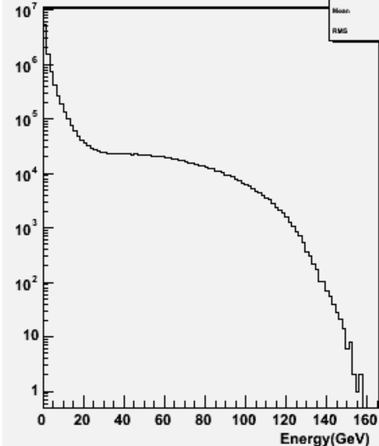
Particle Energy : w100776 e1e1cse1n1_o
