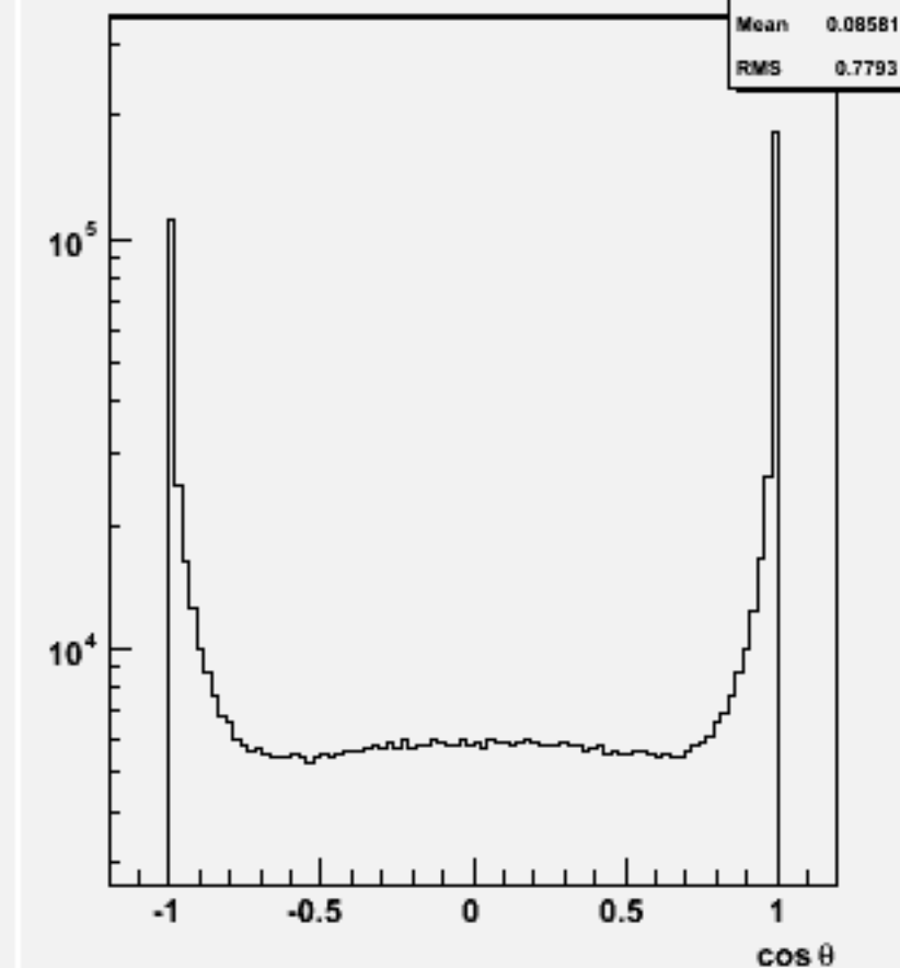
Jet cos \theta (All jets)w100776 e1e1cse1n1_o
