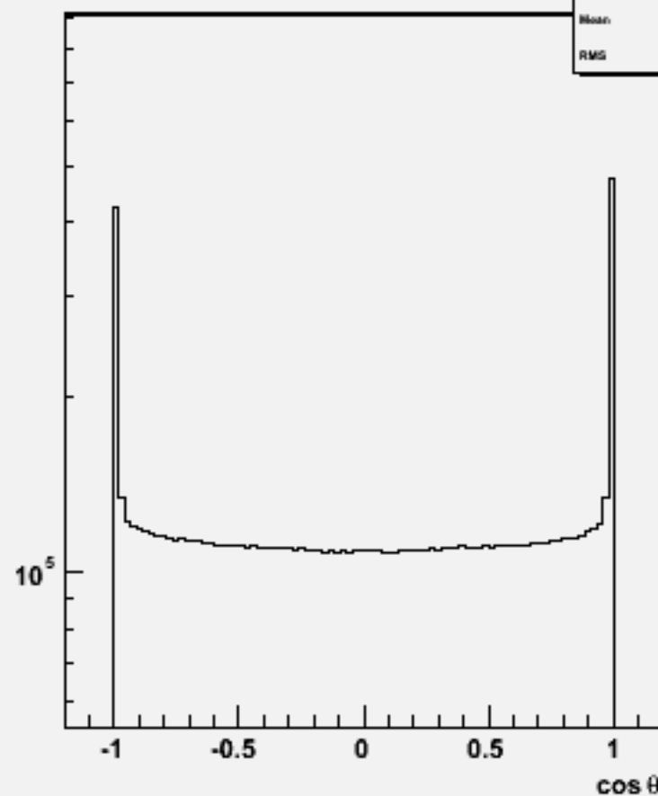
Particle cos \theta : w100776 e1e1cse1n1_o
