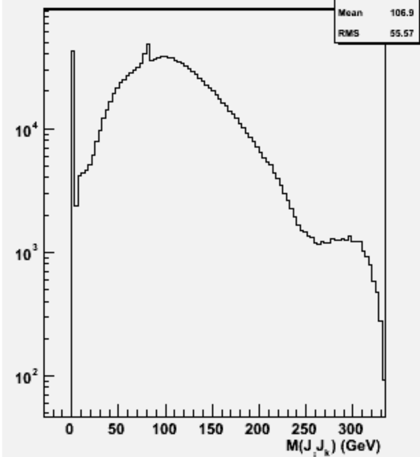
2jets mass(All comb)w100776 e1e1cse1n1_o
