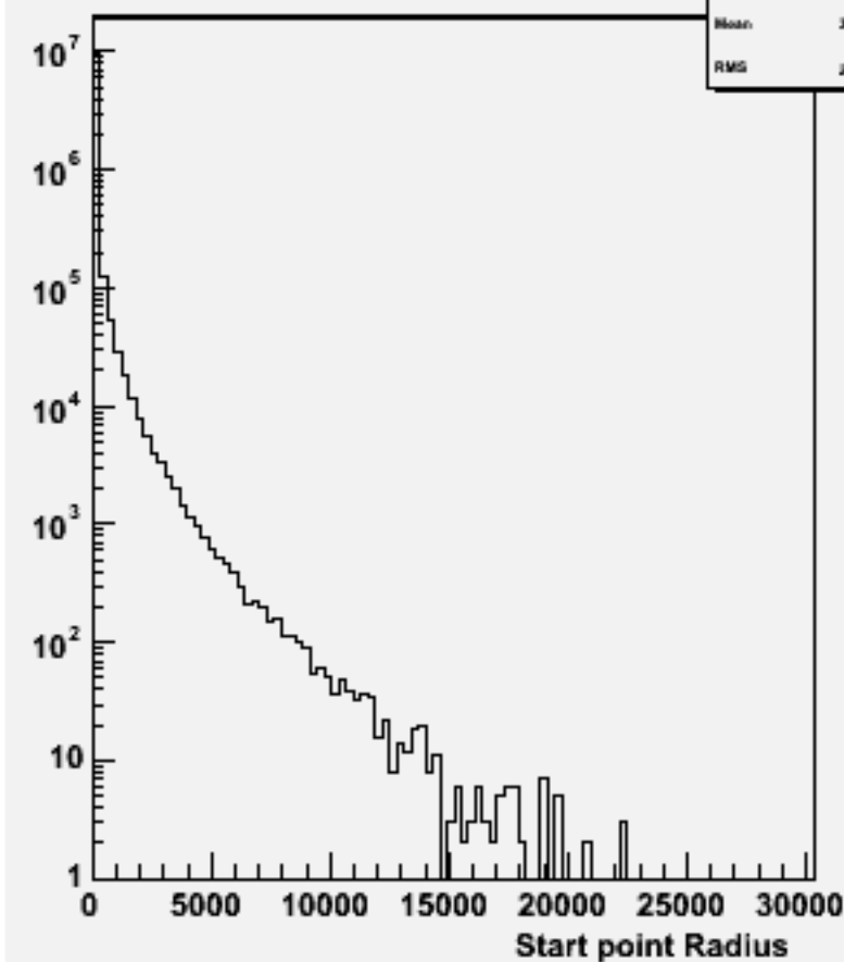
Start point R : w100776 e1e1cse1n1_o
