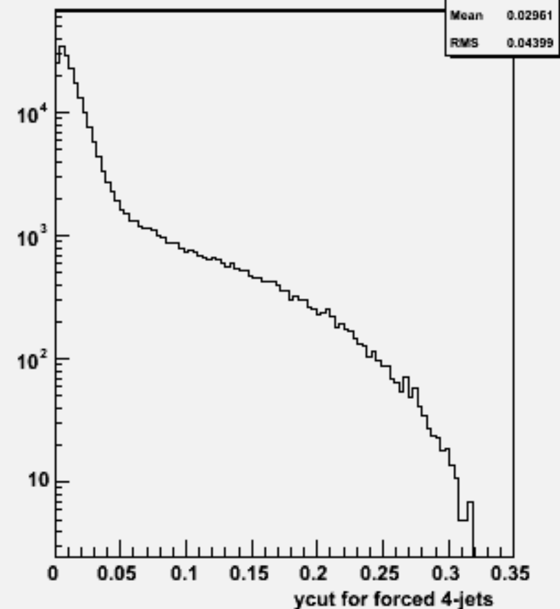
Ycut for 4-jets :w100776 e1e1cse1n1_o
