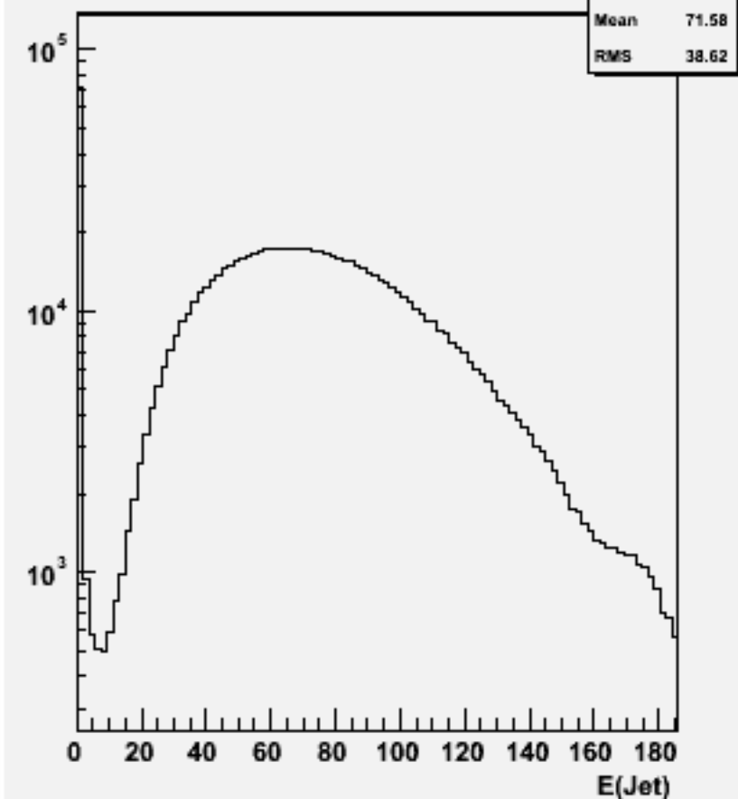
Jet energies(All jets)w100776 e1e1cse1n1_o
