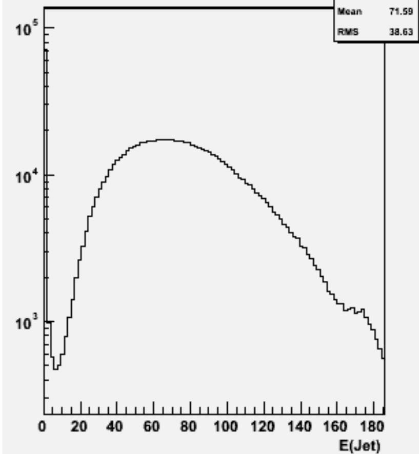
Jet energies(All jets)w100775 e1e1cse1n1_o
