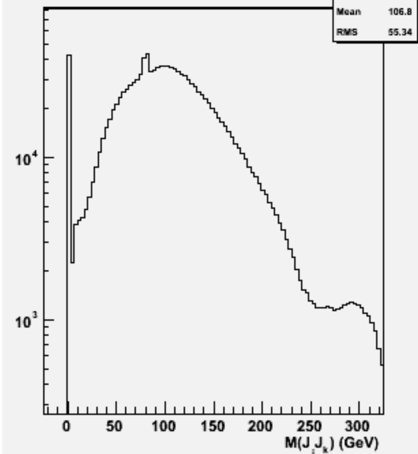
2jets mass(All comb)w100775 e1e1cse1n1_o
