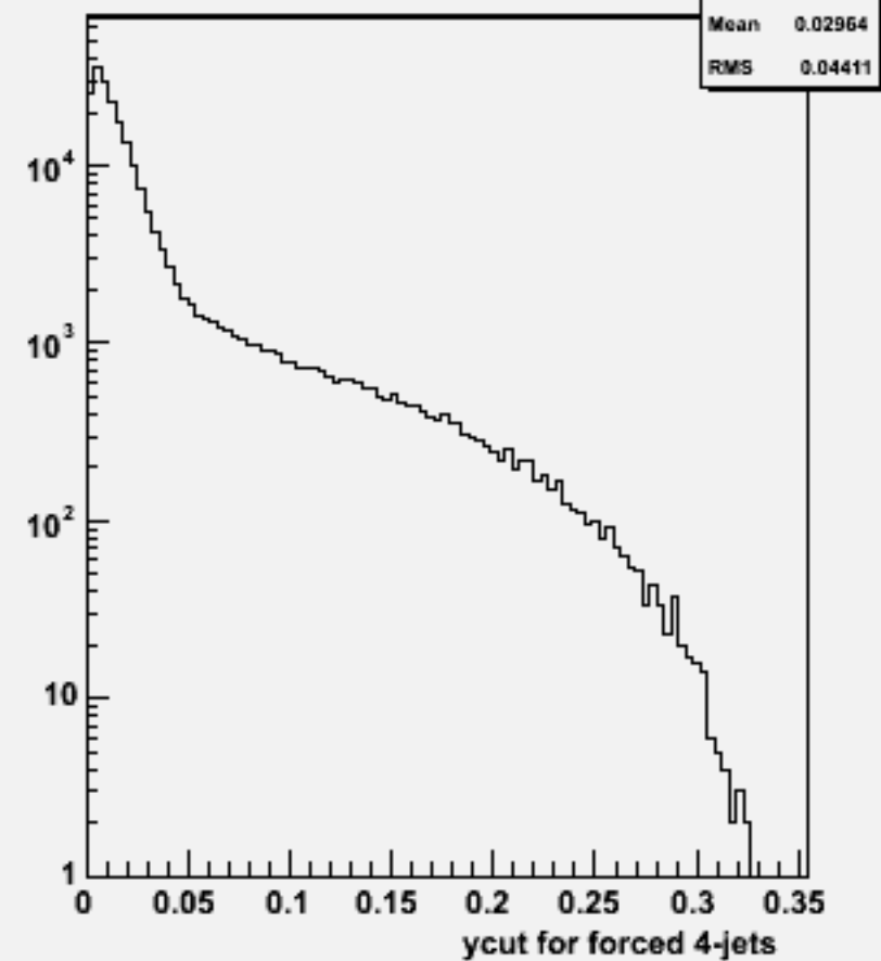
Ycut for 4-jets :w100775 e1e1cse1n1_o
