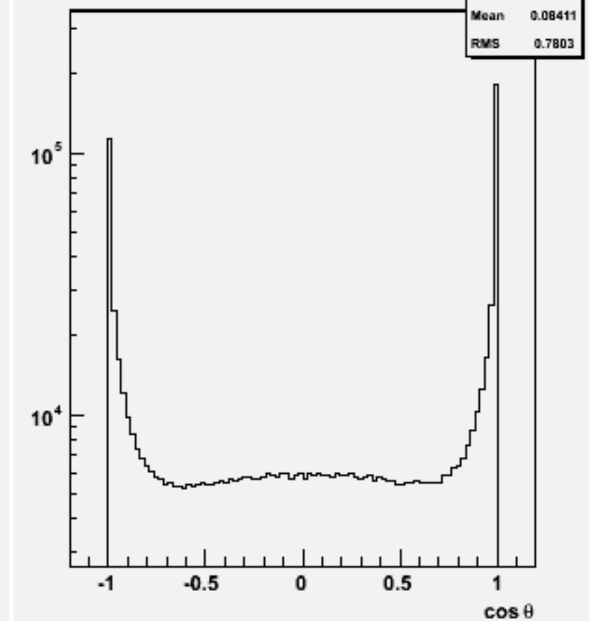
Jet cos \theta (All jets)w100775 e1e1cse1n1_o
