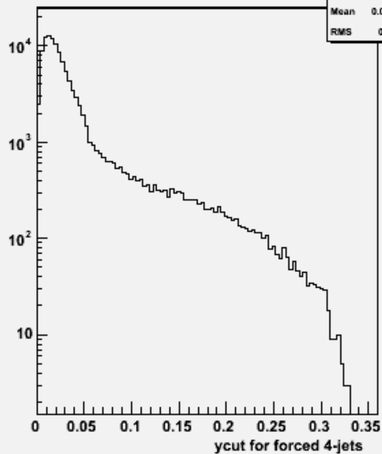
Ycut for 4-jets :w100773 e1e1udsc_o
