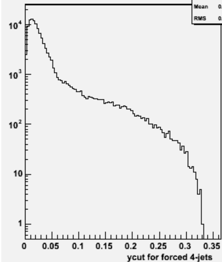
Ycut for 4-jets :w100771 e1e1udsc_o
