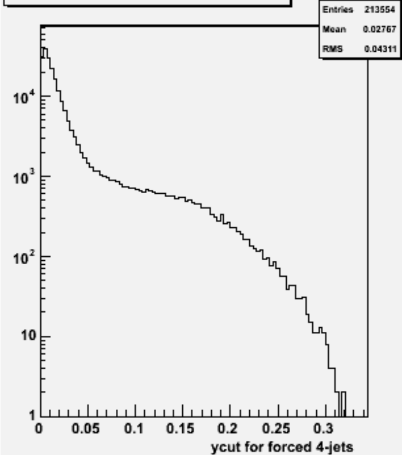
Ycut for 4-jets :w100766 e1e1ude3n3_o
