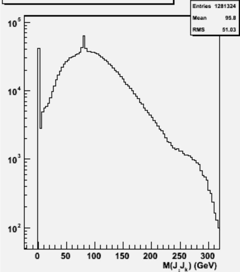
2jets mass(All comb)w100766 e1e1ude3n3_o
