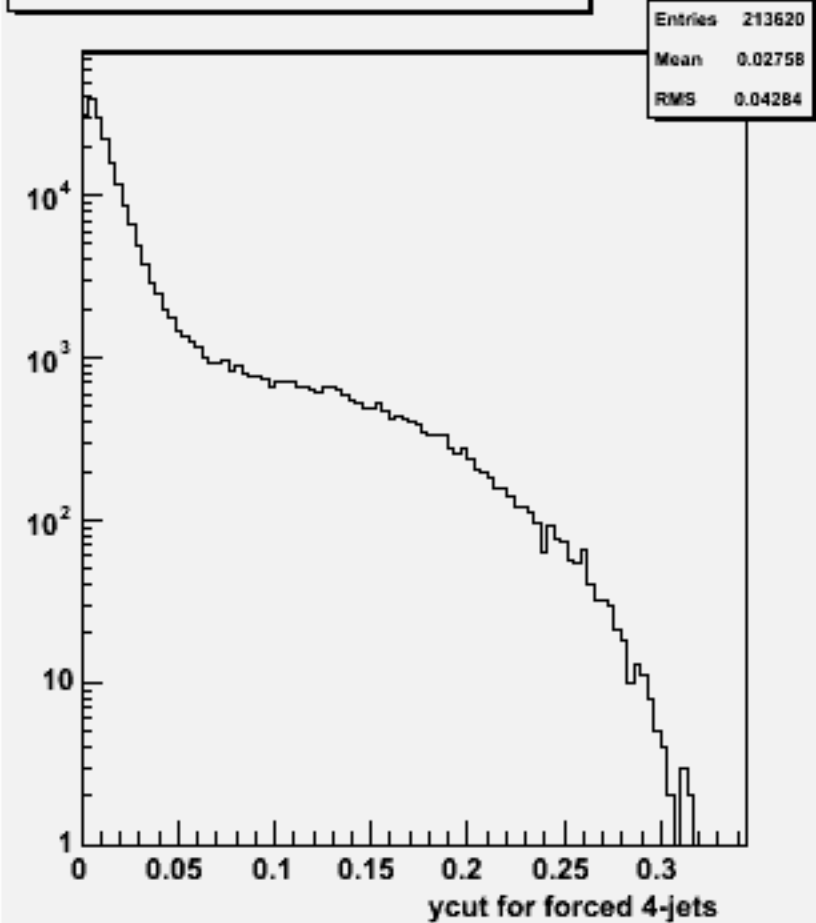
Ycut for 4-jets :w100765 e1e1ude3n3_o
