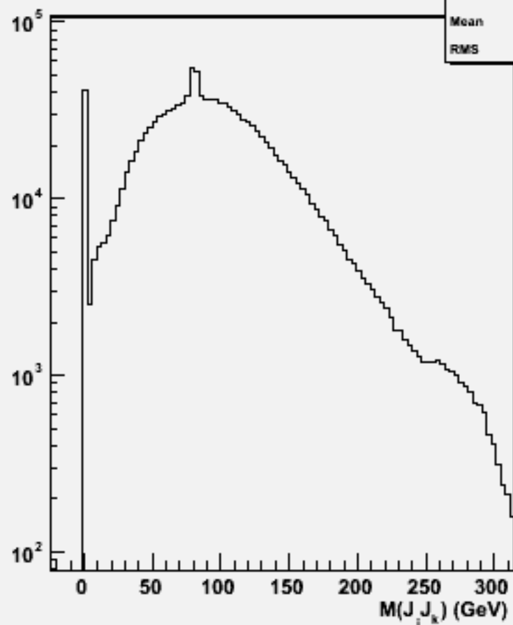
2jets mass(All comb)w100763 e1e1ude3n3_o
