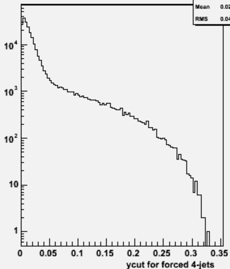
Ycut for 4-jets :w100762 e1e1ude2n2_o
