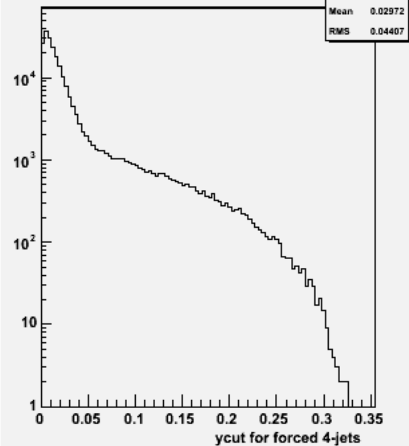
Ycut for 4-jets :w100761 e1e1ude2n2_o
