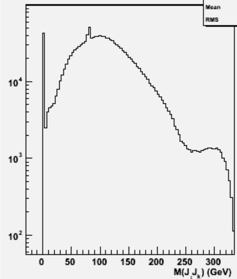
2jets mass(All comb)w100759 e1e1ude2n2_o
