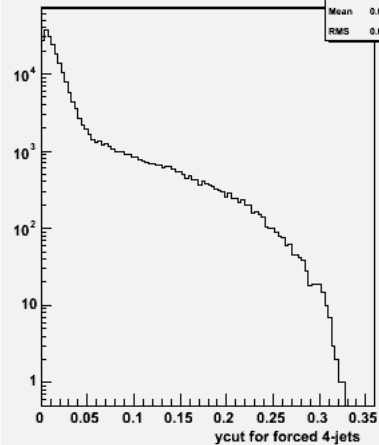
Ycut for 4-jets :w100759 e1e1ude2n2_o
