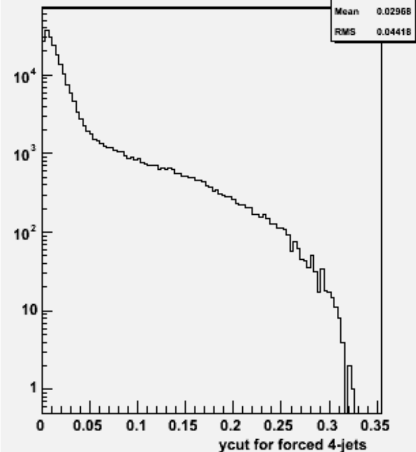
Ycut for 4-jets :w100758 e1e1ude1n1_o
