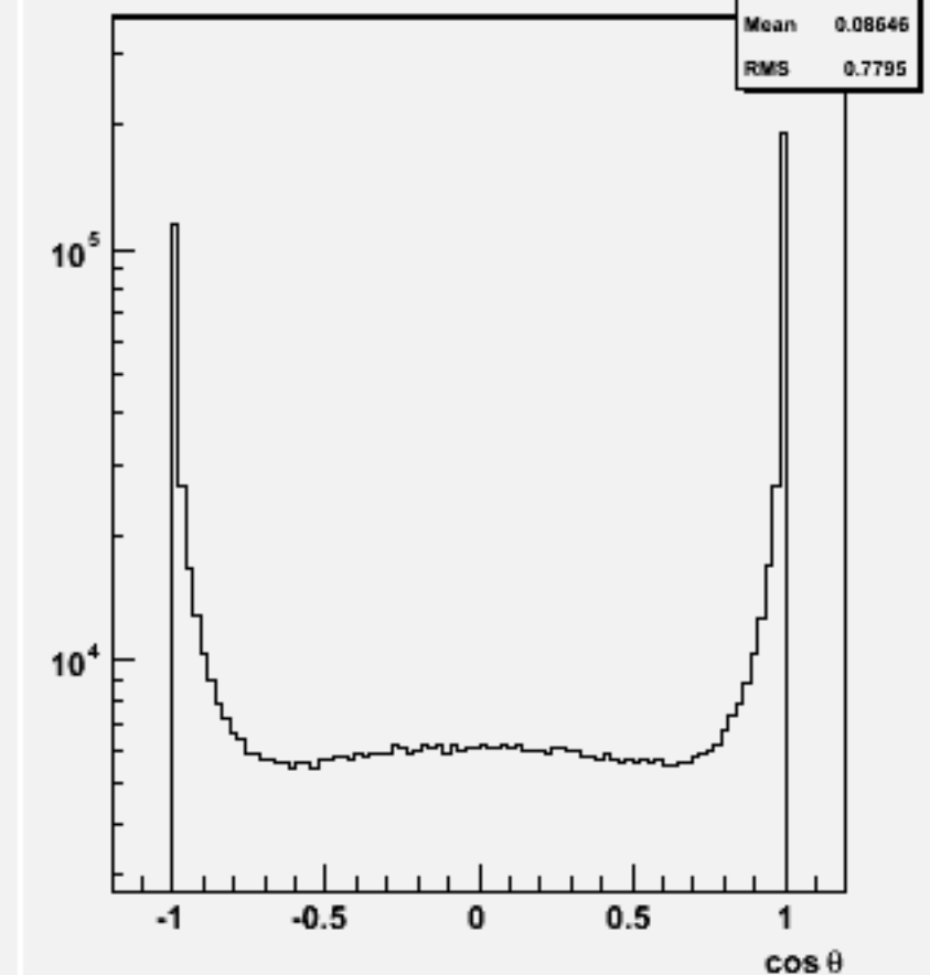
Jet cos \theta (All jets)w100758 e1e1ude1n1_o
