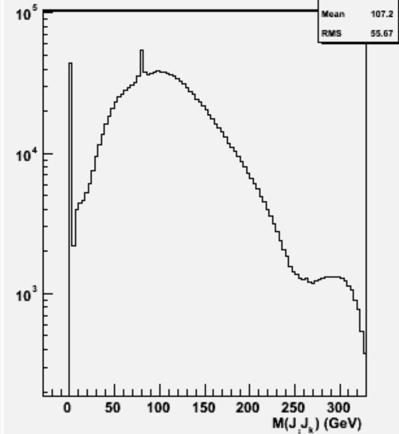
2jets mass(All comb)w100758 e1e1ude1n1_o
