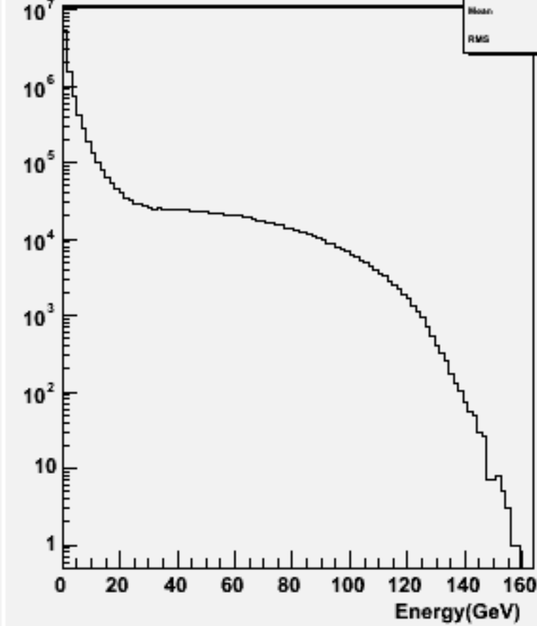
Particle Energy : w100758 e1e1ude1n1_o
