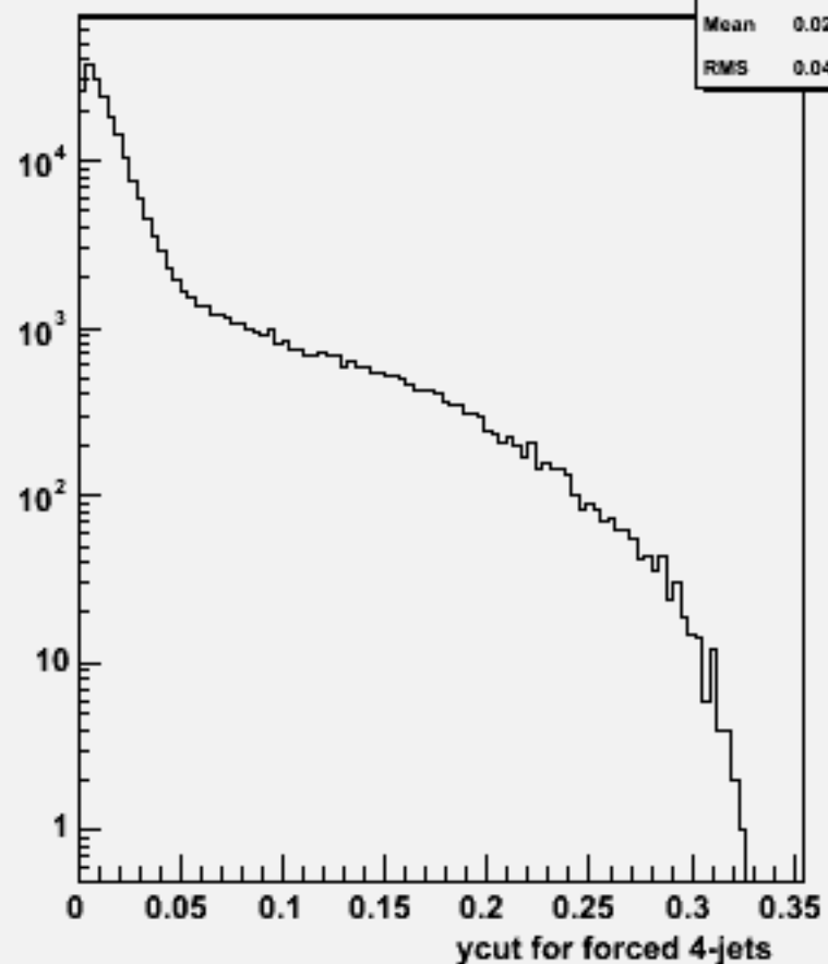
Ycut for 4-jets :w100757 e1e1ude1n1_o
