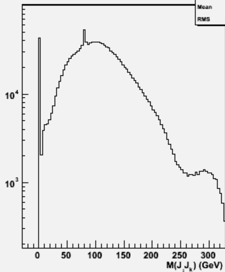
2jets mass(All comb)w100757 e1e1ude1n1_o
