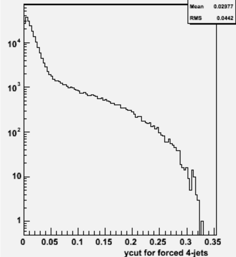
Ycut for 4-jets :w100756 e1e1ude1n1_o
