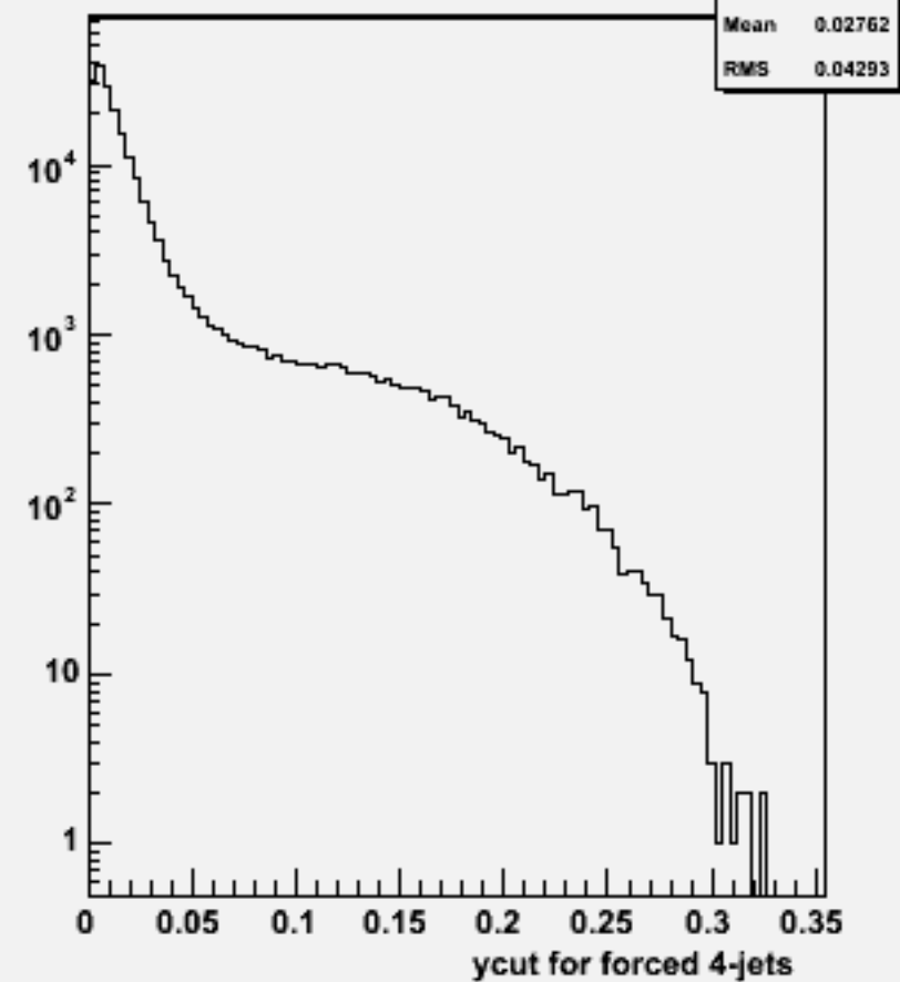
Ycut for 4-jets :w100754 e1e1n3e3sc_o
