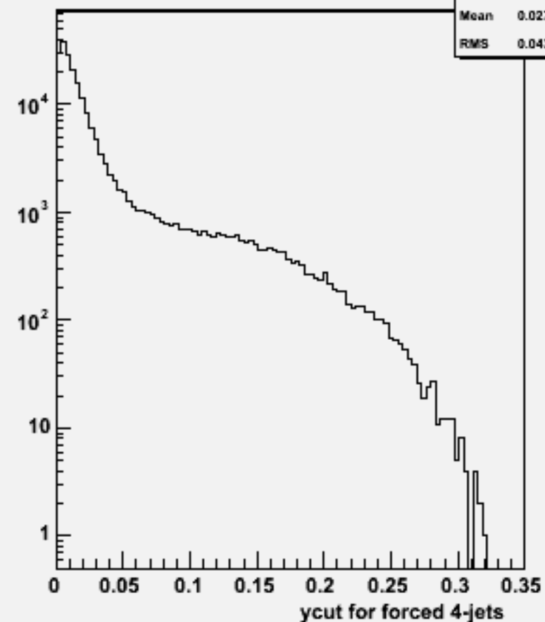
Ycut for 4-jets :w100752 e1e1n3e3sc_o
