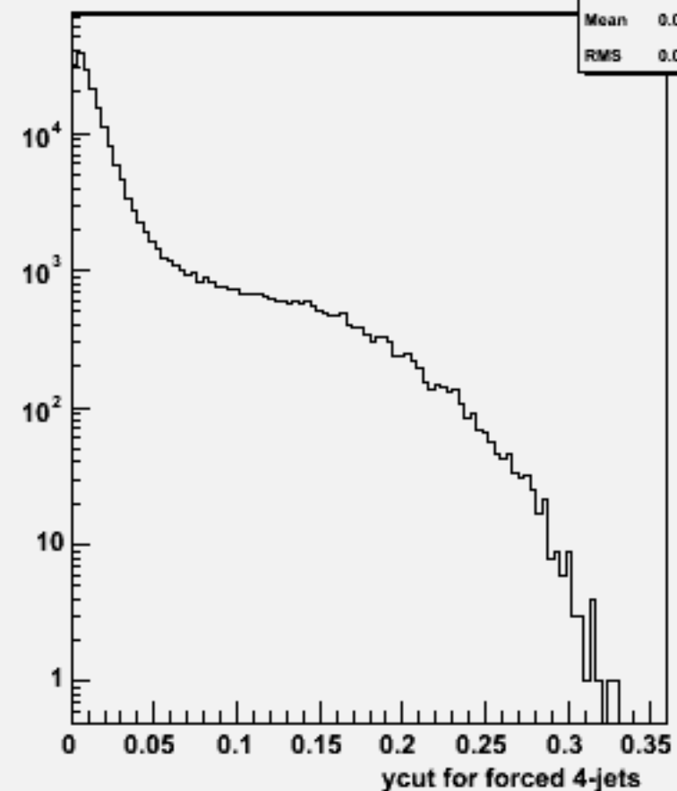
Ycut for 4-jets :w100751 e1e1n3e3sc_o
