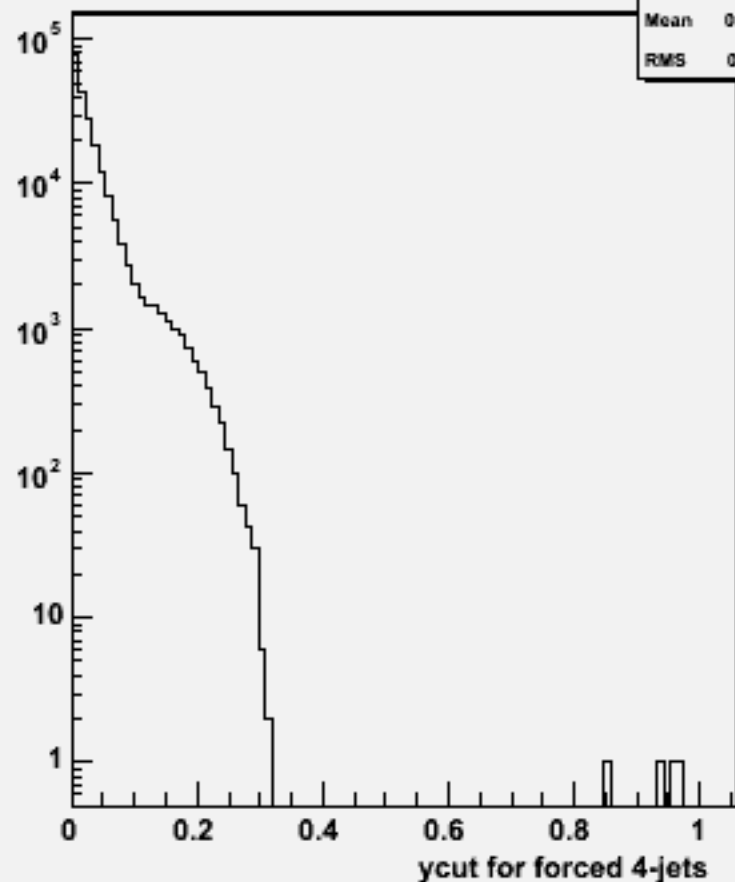
Ycut for 4-jets :w100738 e1e1n3e3e1n1_o
