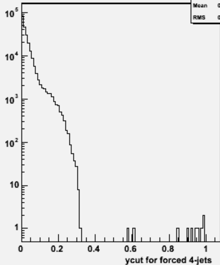
Ycut for 4-jets :w100736 e1e1n3e3e1n1_o
