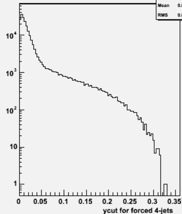
Ycut for 4-jets :w100712 e1e1n1e1sc_o
