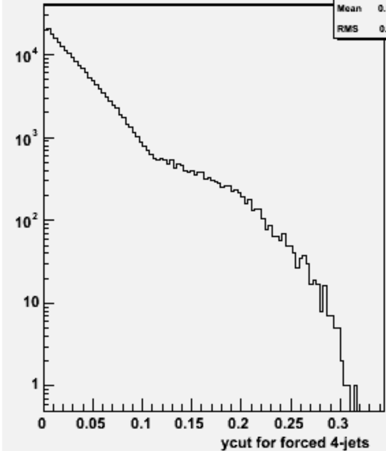
Ycut for 4-jets :w100698 e1e1n1e1e1n1_o
