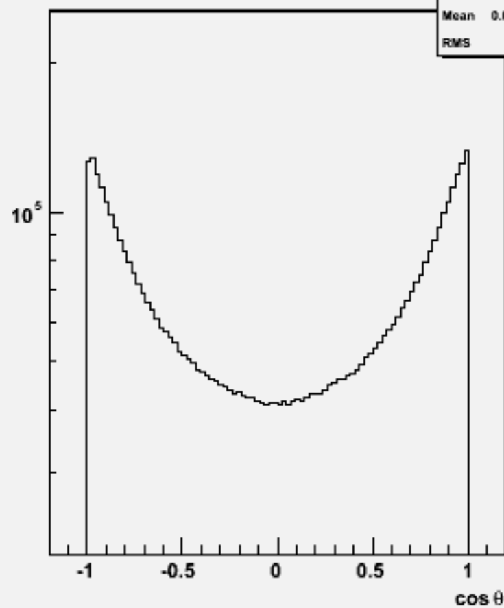
Particle cos \theta : w100692 bbbb_o
