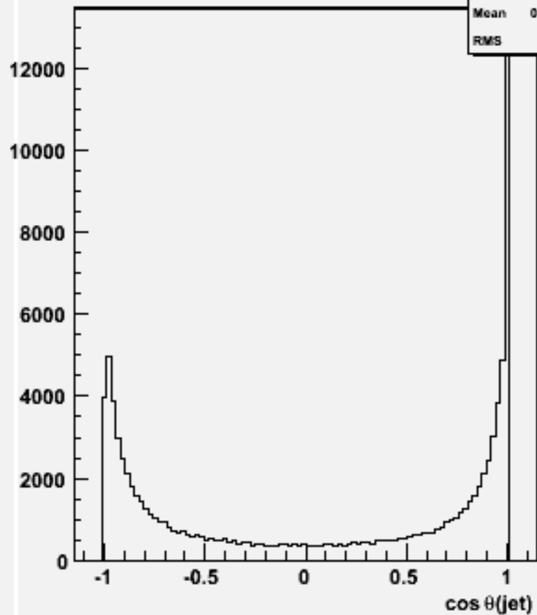
cos \theta for 2-jets :w100692 bbbb_o
