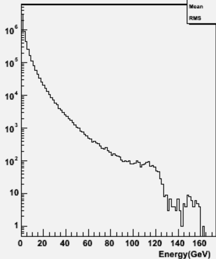
Particle Energy : w100692 bbbb_o
