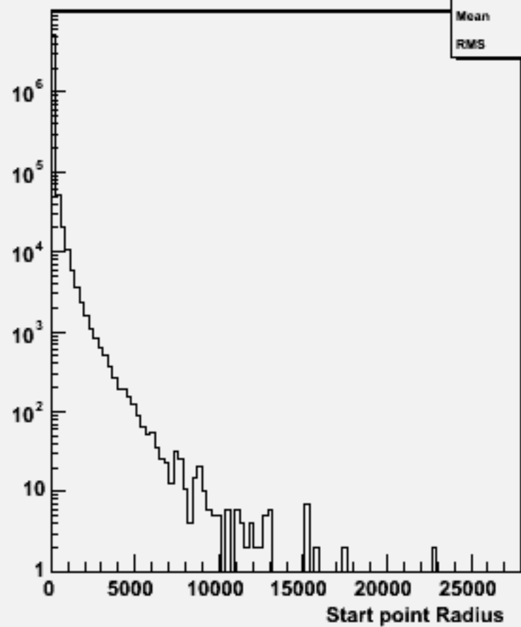
Start point R : w100692 bbbb_o
