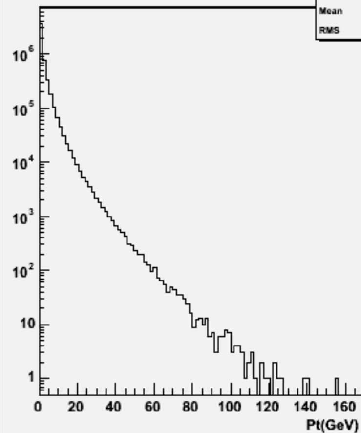
Particle Pt : w100692 bbbb_o
