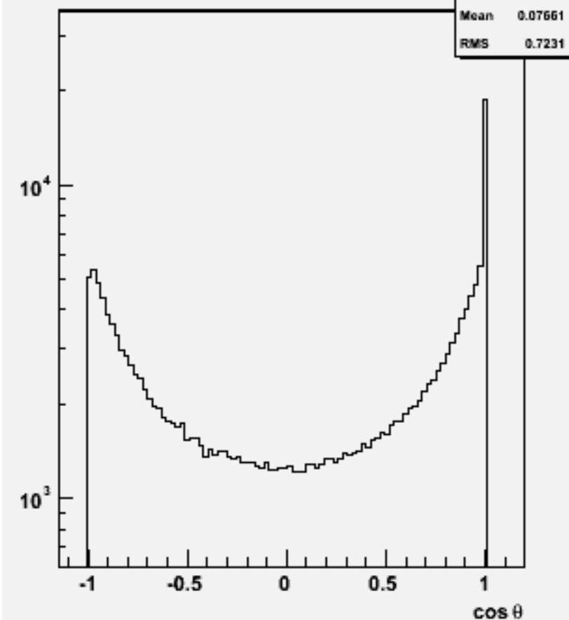
Jet cos \theta (All jets)w100692 bbbb_o
