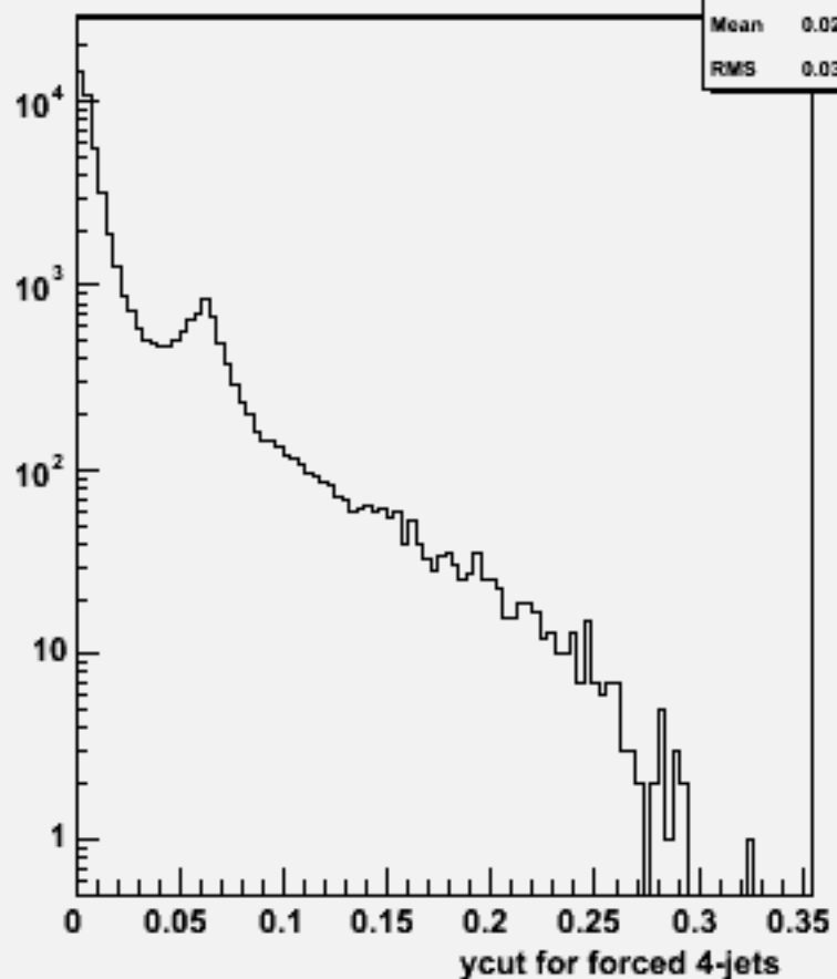
Ycut for 4-jets :w100692 bbbb_o
