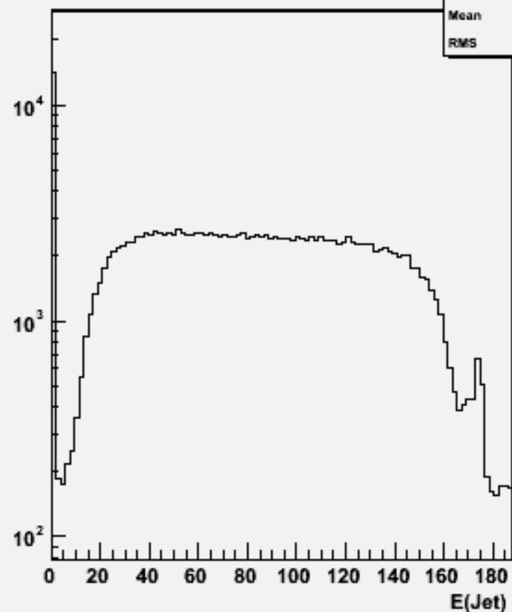
Jet energies(All jets)w100692 bbbb_o
