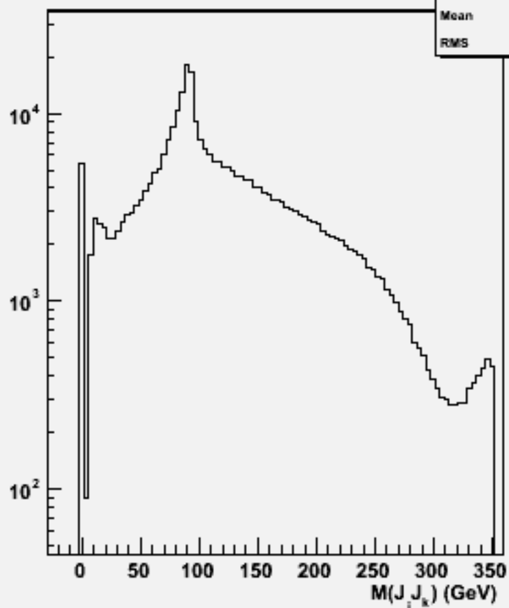
2jets mass(All comb)w100692 bbbb_o
