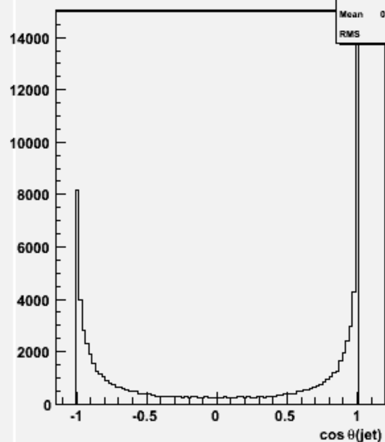
cos \theta for 2-jets :w100677 ddss_o
