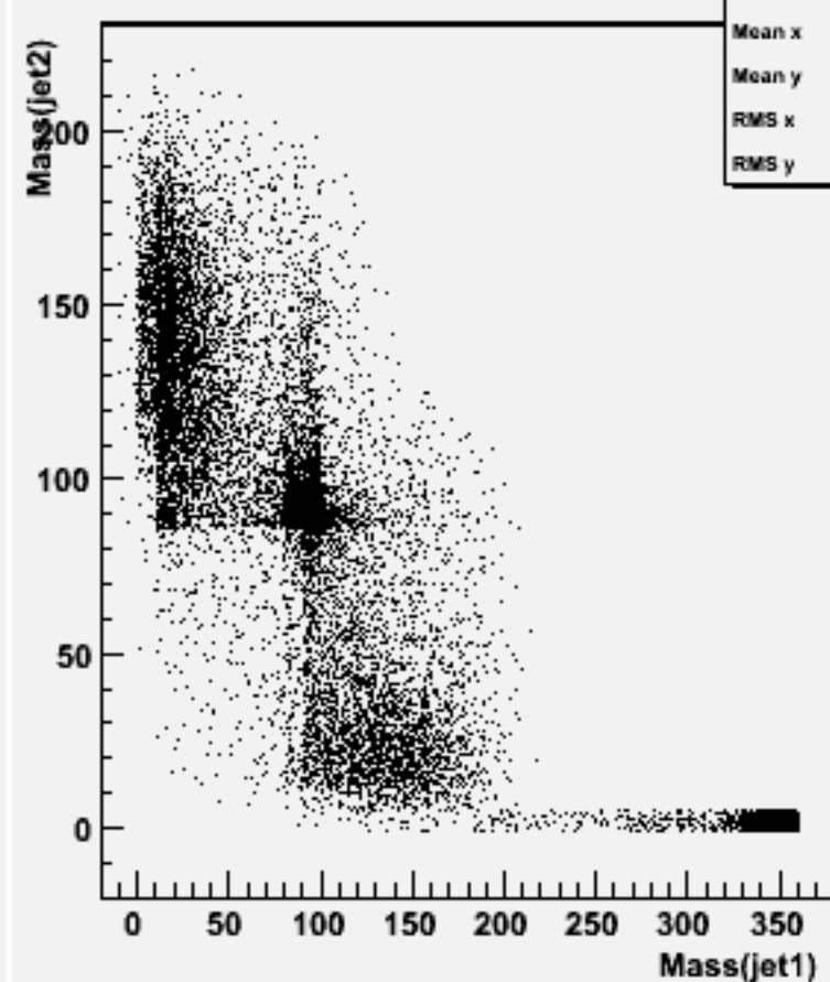
Jet mass for forced 2-jets : w100677 ddss_o
