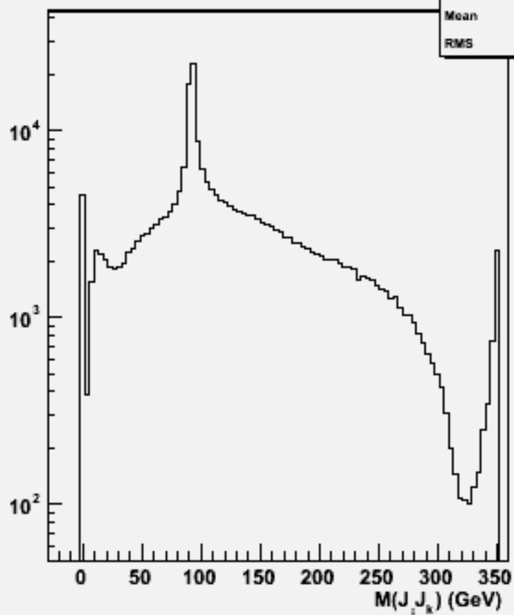
2jets mass(All comb)w100677 ddss_o
