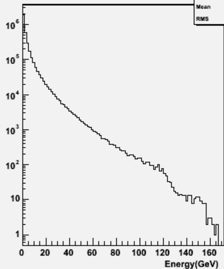
Particle Energy : w100677 ddss_o
