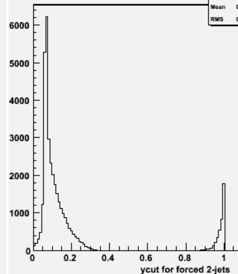
Ycut for 2-jets :w100677 ddss_o
