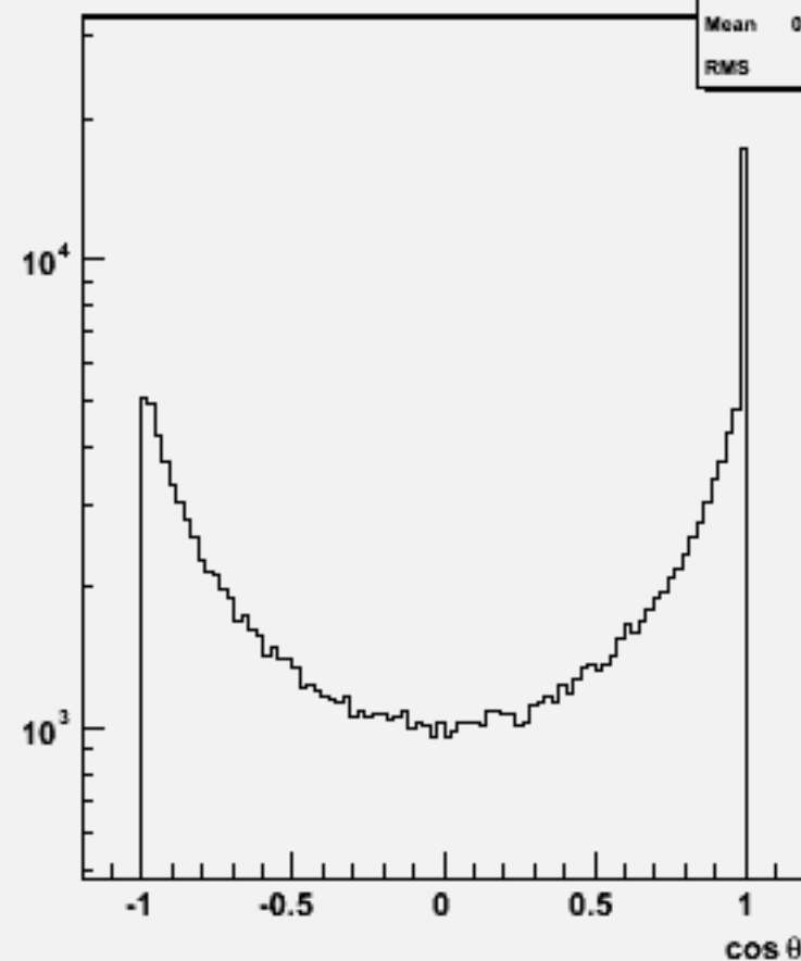
Jet cos \theta (All jets)w100677 ddss_o
