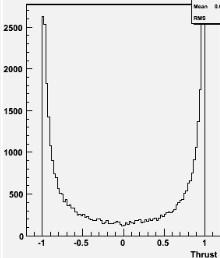
cos \Theta (thrust) w100677 ddss_o
