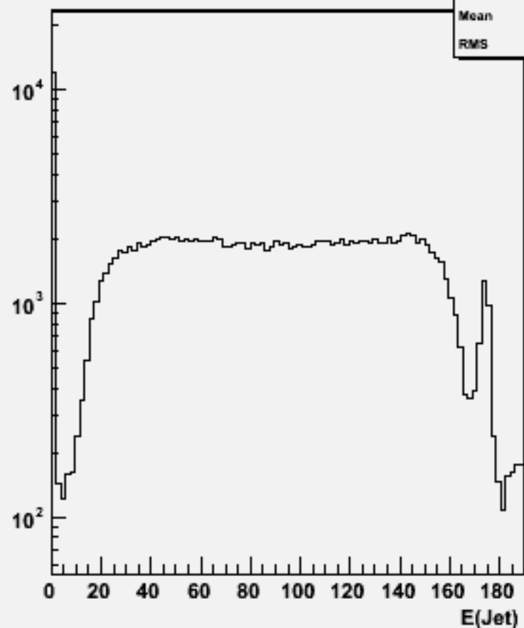
Jet energies(All jets)w100677 ddss_o
