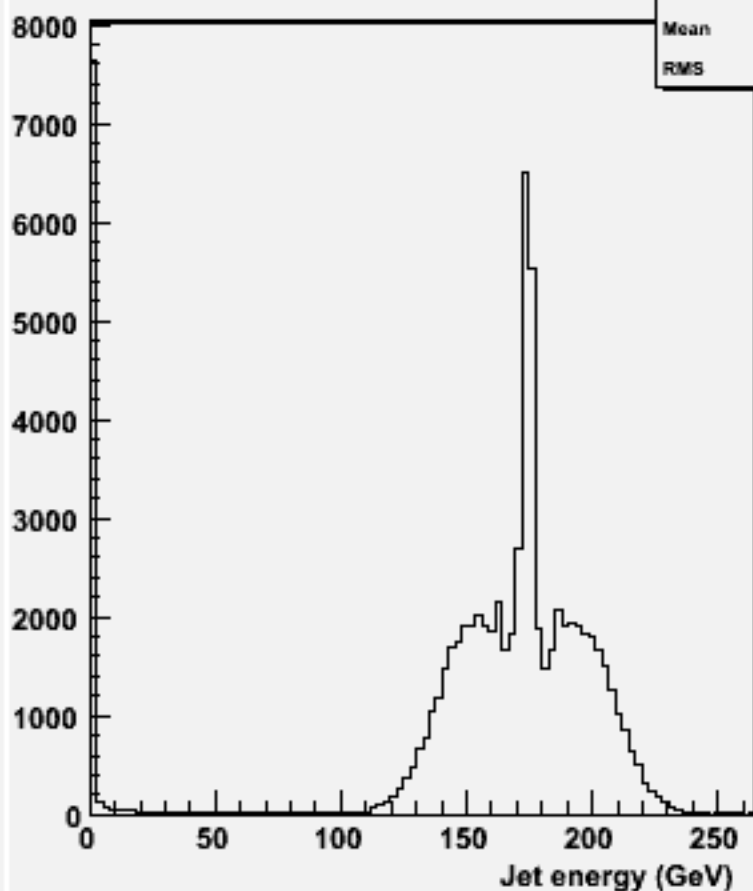
energy for 2-jets :w100677 ddss_o
