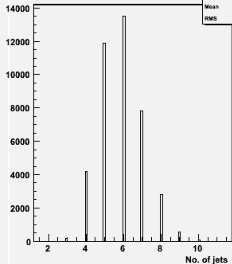
No. jets (ycut=0.001) : w100677 ddss_o
