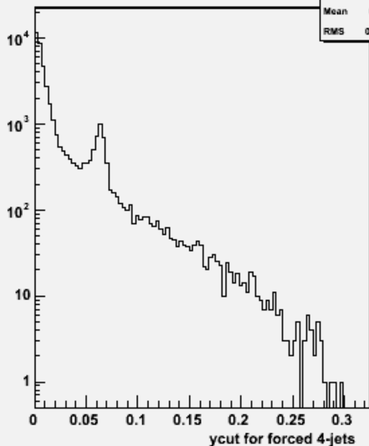
Ycut for 4-jets :w100677 ddss_o
