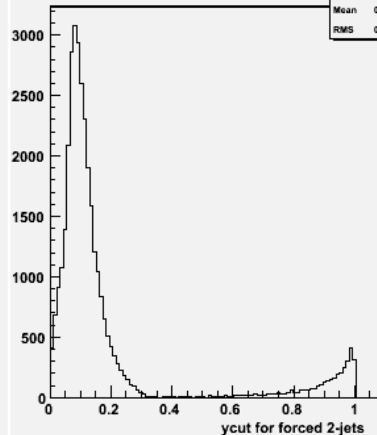
Ycut for 2-jets :w100668 e3e3bb_o
