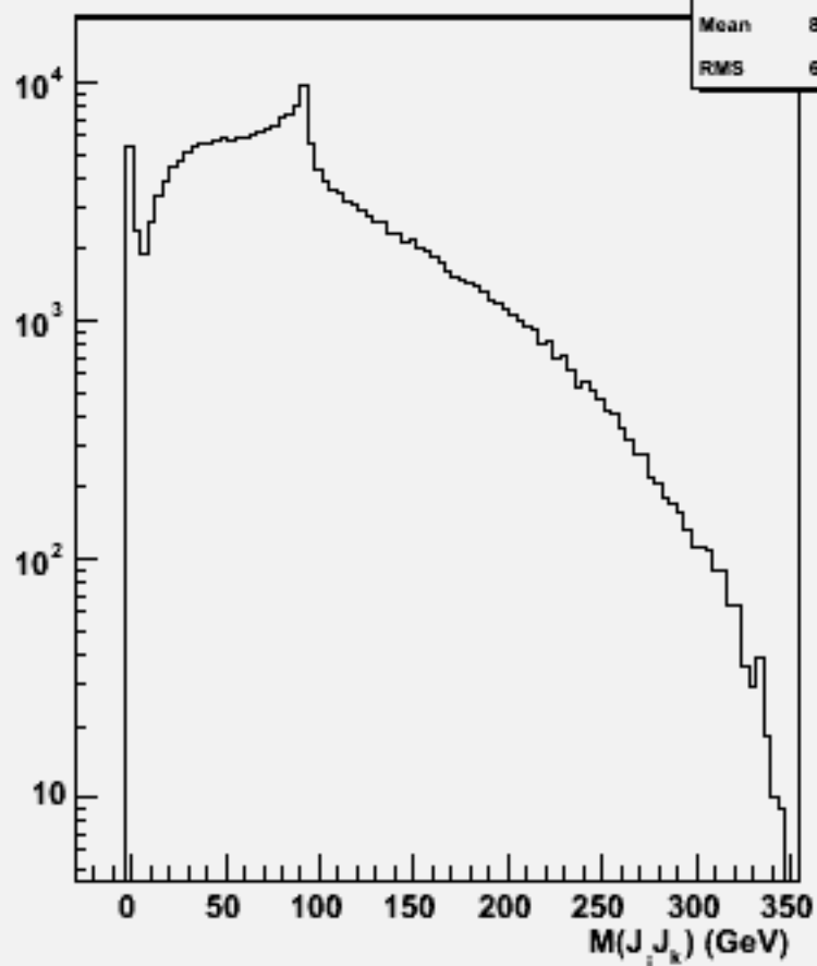
2jets mass(All comb)w100668 e3e3bb_o
