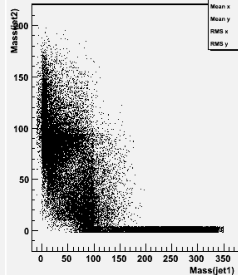
Jet mass for forced 2-jets : w100668 e3e3bb_o
