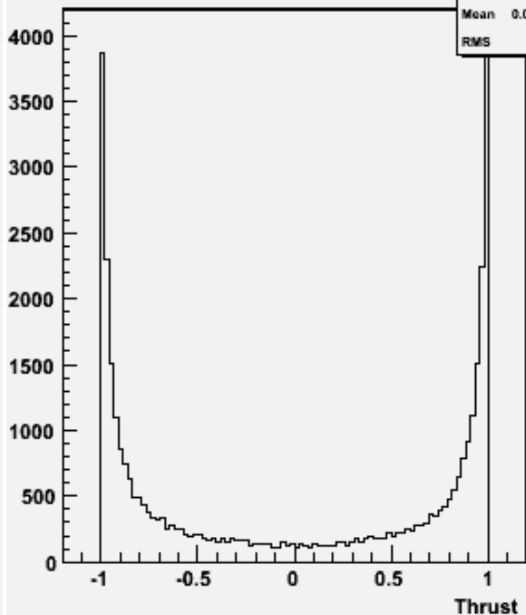
cos \Theta (thrust) w100668 e3e3bb_o
