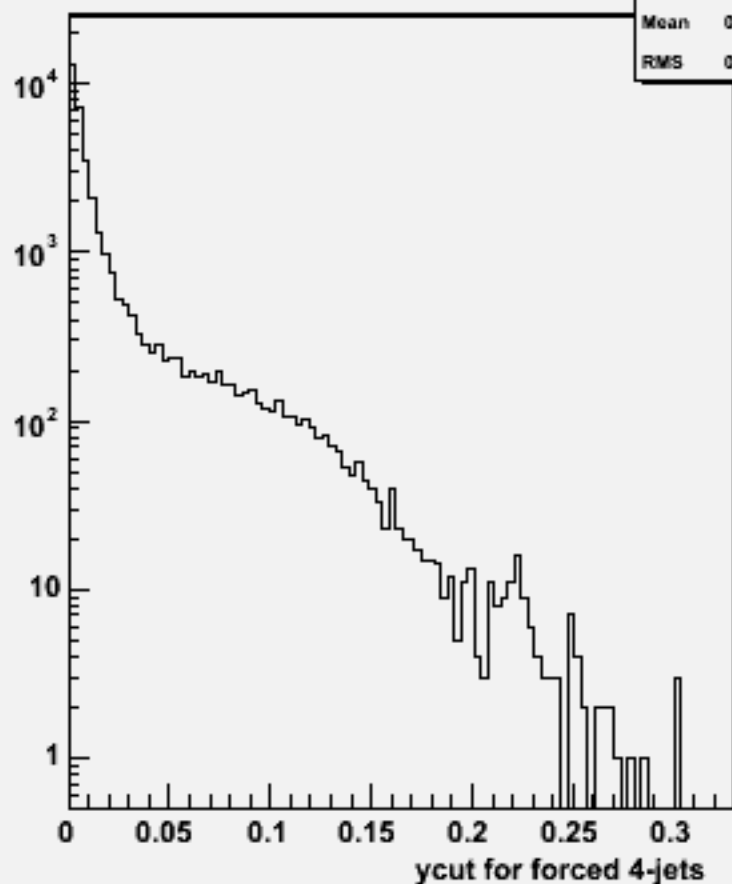
Ycut for 4-jets :w100668 e3e3bb_o
