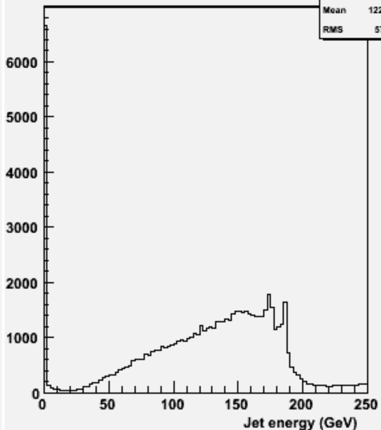
energy for 2-jets :w100668 e3e3bb_o
