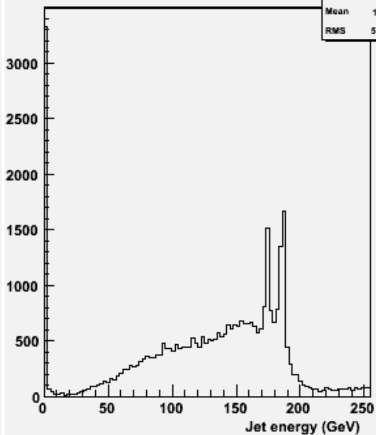
energy for 2-jets :w100661 e3e3dd_o
