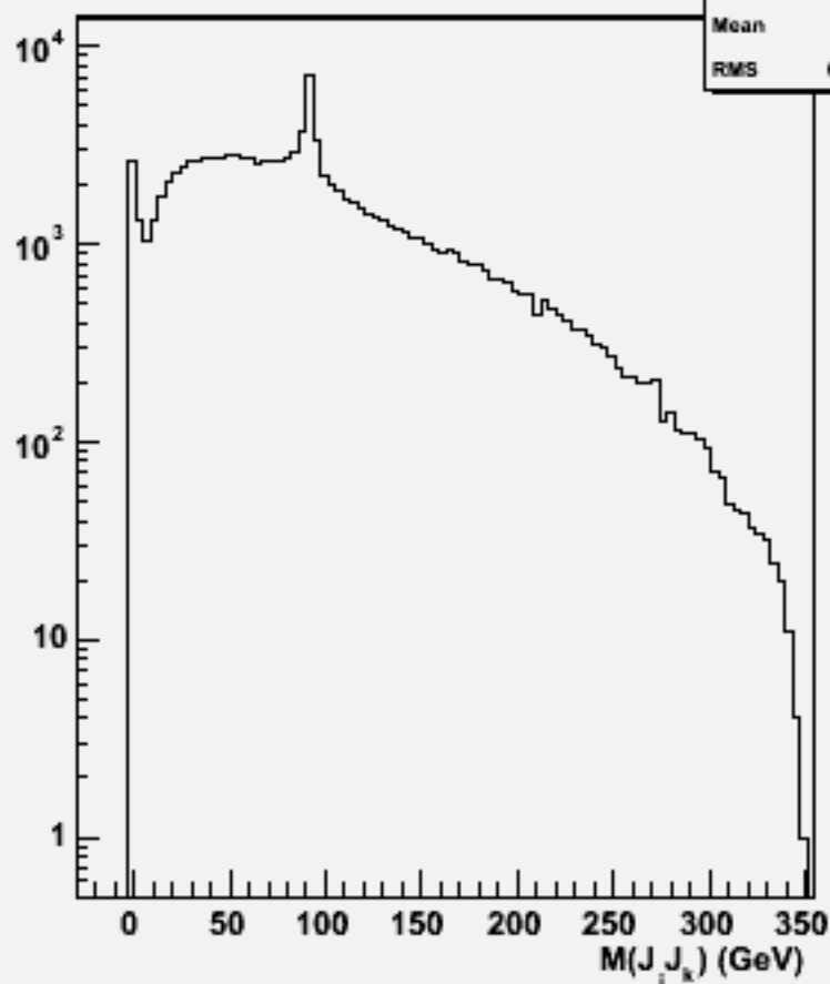
2jets mass(All comb)w100661 e3e3dd_o
