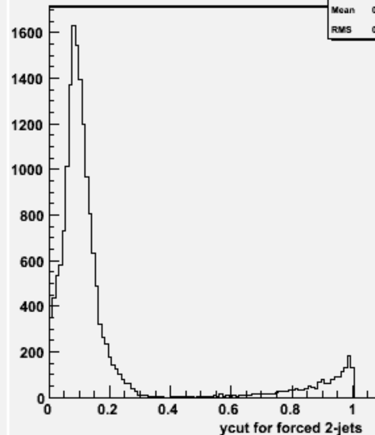
Ycut for 2-jets :w100661 e3e3dd_o
