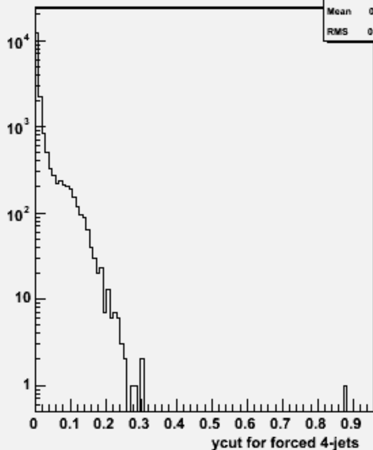
Ycut for 4-jets :w100661 e3e3dd_o
