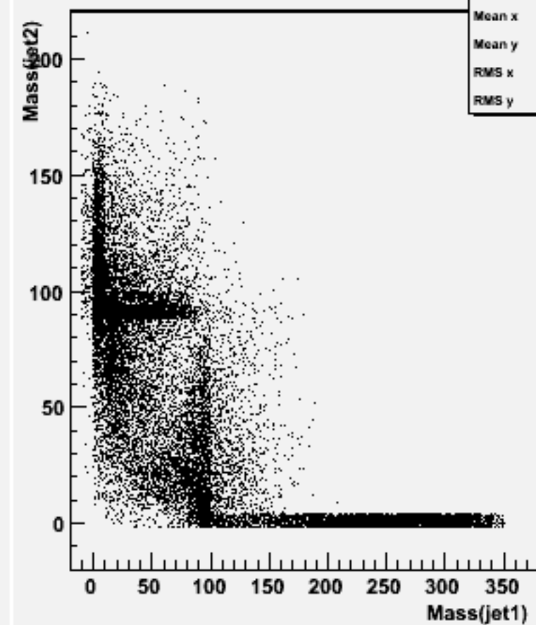
Jet mass for forced 2-jets : w100661 e3e3dd_o
