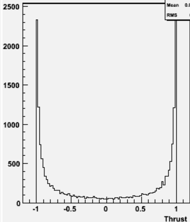
cos \Theta (thrust) w100661 e3e3dd_o
