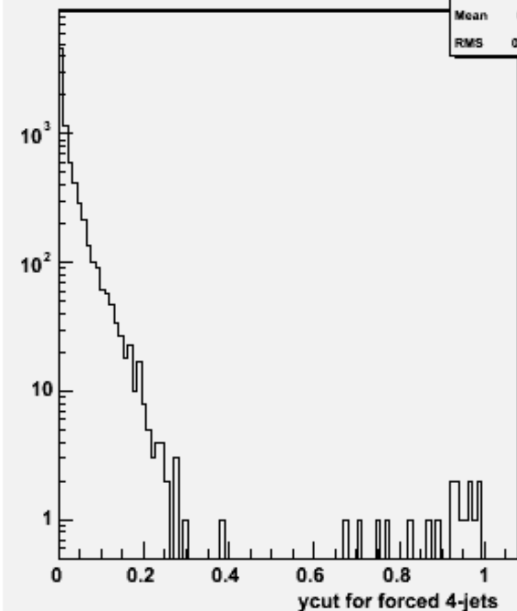
Ycut for 4-jets :w100656 e3e3e3e3_o
