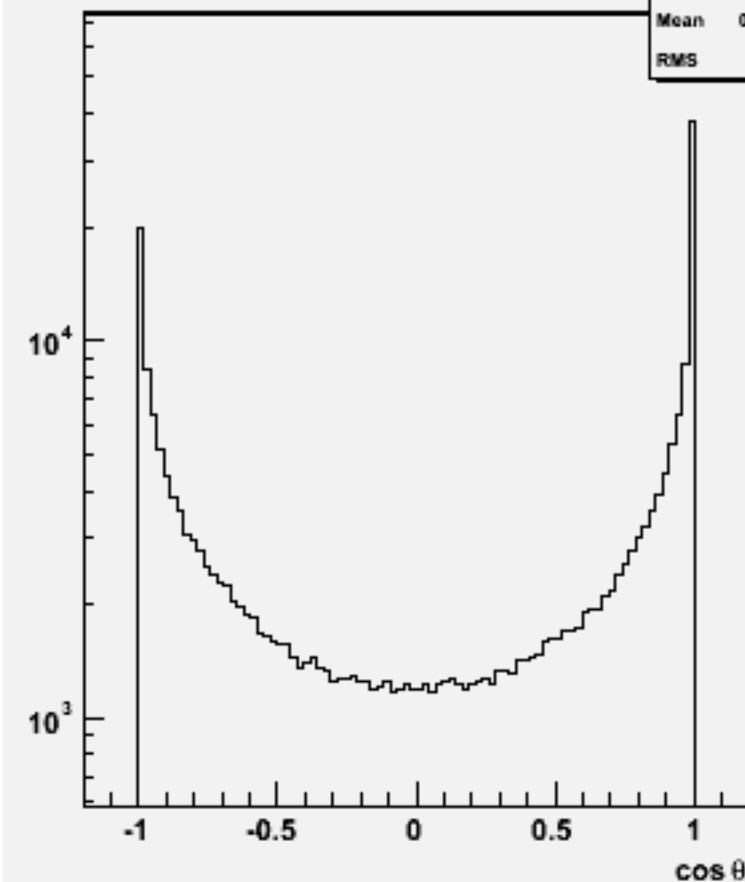
Jet cos \theta (All jets)w100648 e2e2ss_o
