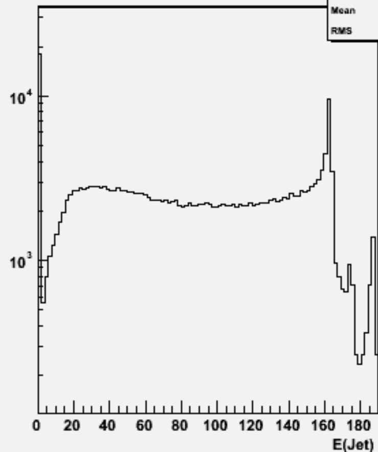
Jet energies(All jets)w100648 e2e2ss_o
