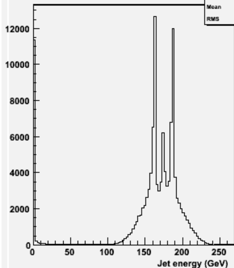
energy for 2-jets :w100648 e2e2ss_o
