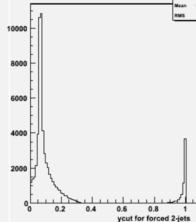
Ycut for 2-jets :w100648 e2e2ss_o
