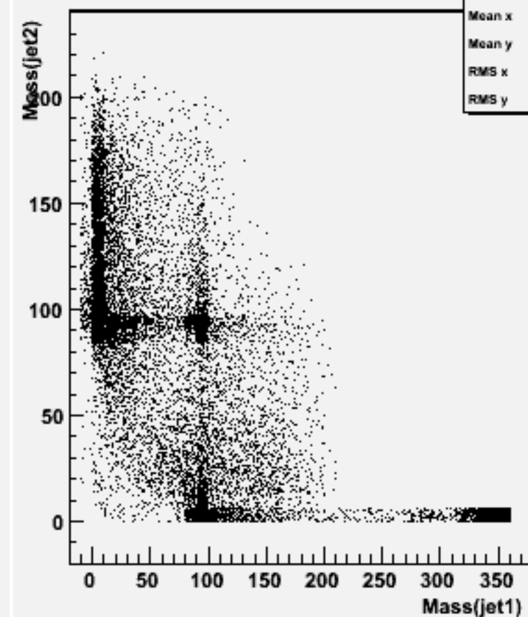
Jet mass for forced 2-jets : w100648 e2e2ss_o
