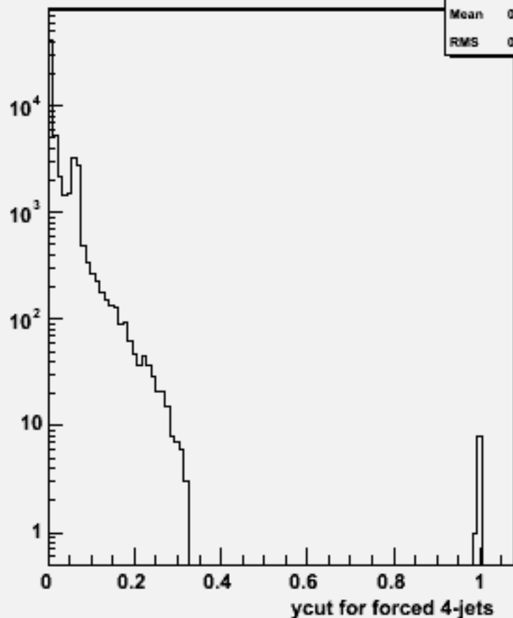
Ycut for 4-jets :w100648 e2e2ss_o
