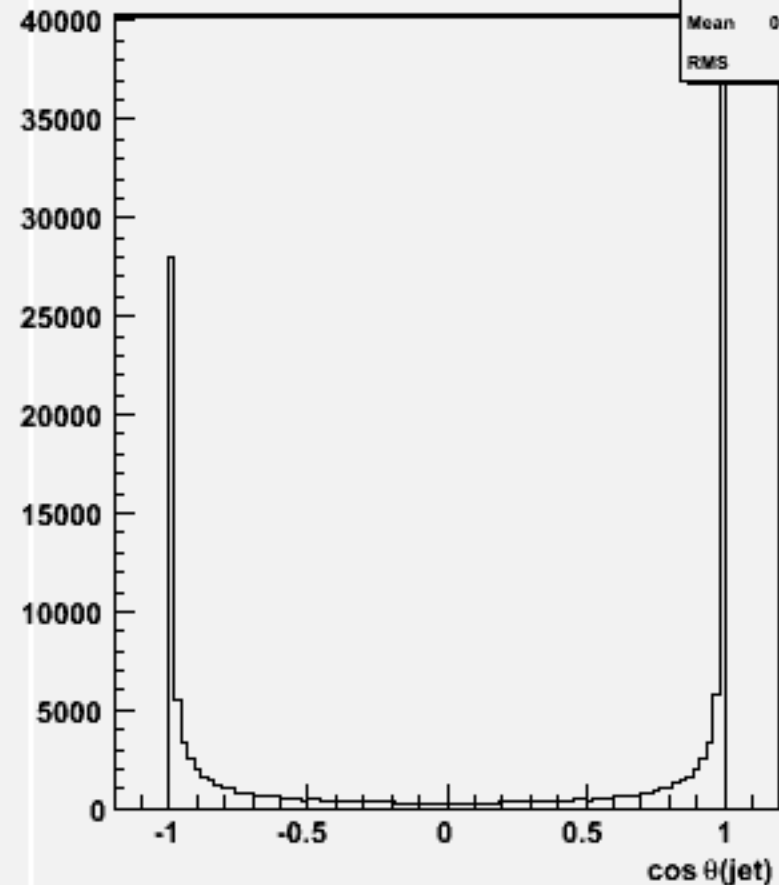
cos \theta for 2-jets :w100648 e2e2ss_o
