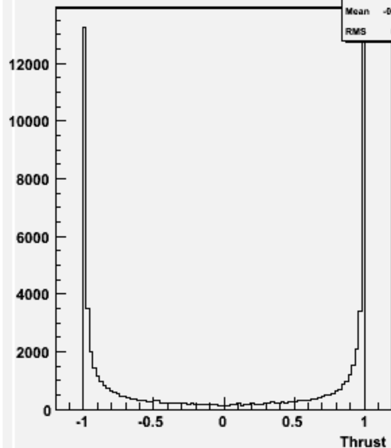
cos \Theta (thrust) w100648 e2e2ss_o
