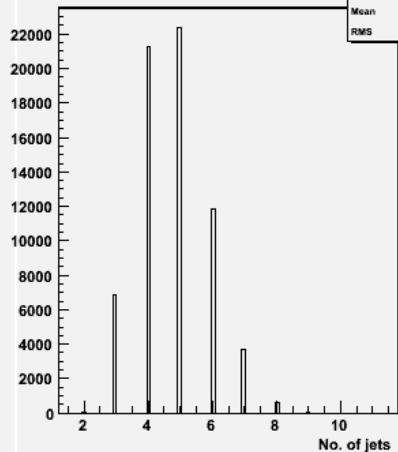
No. jets (ycut=0.001) : w100648 e2e2ss_o
