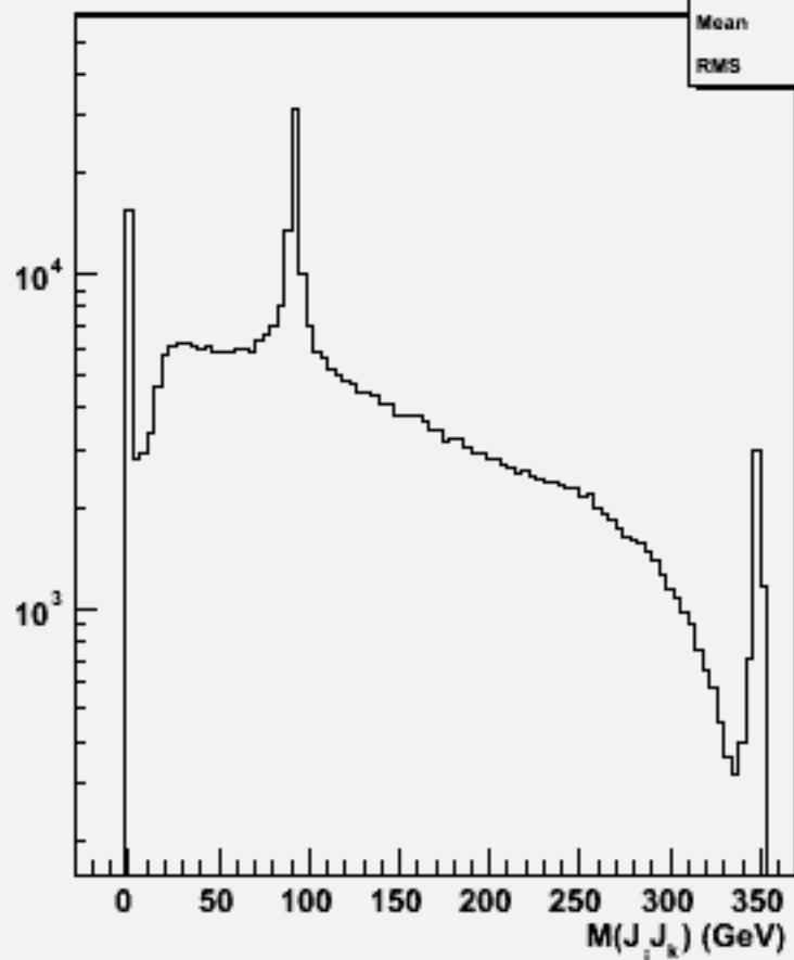
2jets mass(All comb)w100648 e2e2ss_o
