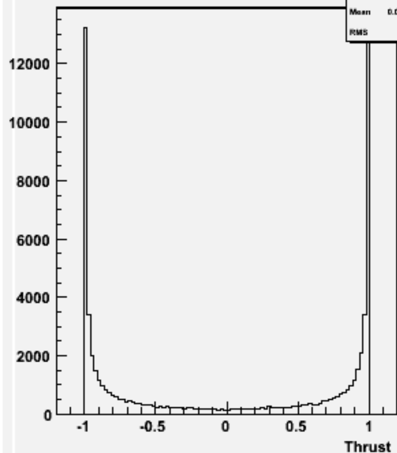
cos \Theta (thrust) w100644 e2e2dd_o
