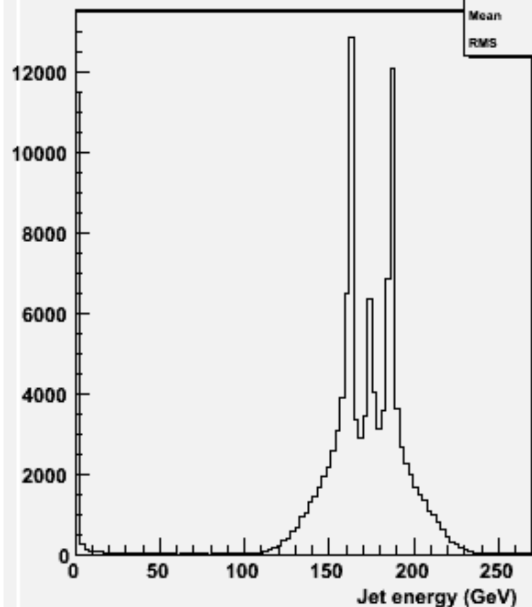
energy for 2-jets :w100644 e2e2dd_o
