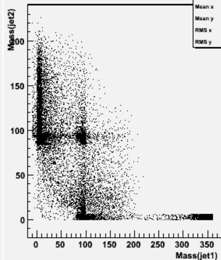
Jet mass for forced 2-jets : w100644 e2e2dd_o
