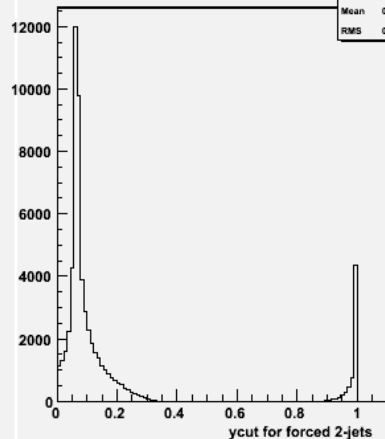
Ycut for 2-jets :w100644 e2e2dd_o
