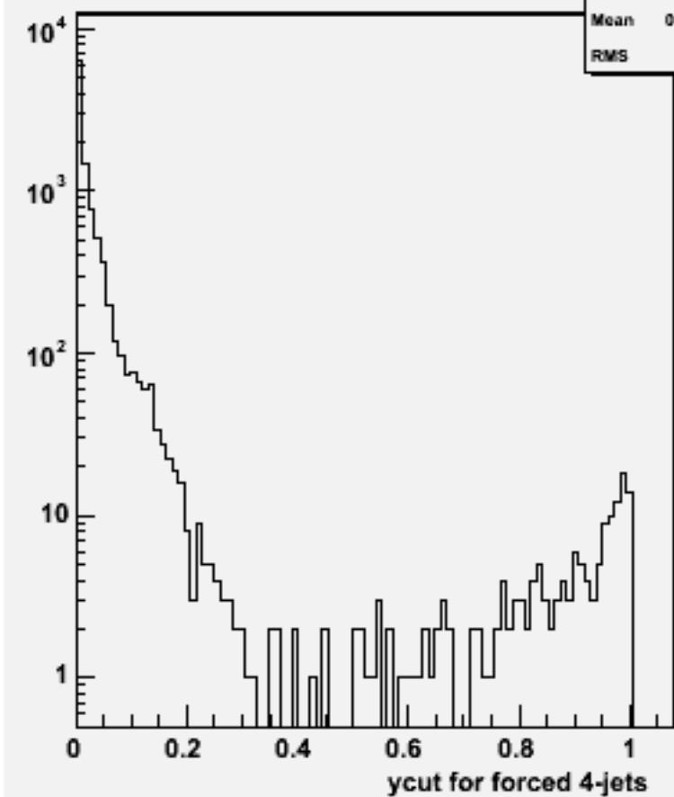
Ycut for 4-jets :w100641 e2e2e3e3_o
