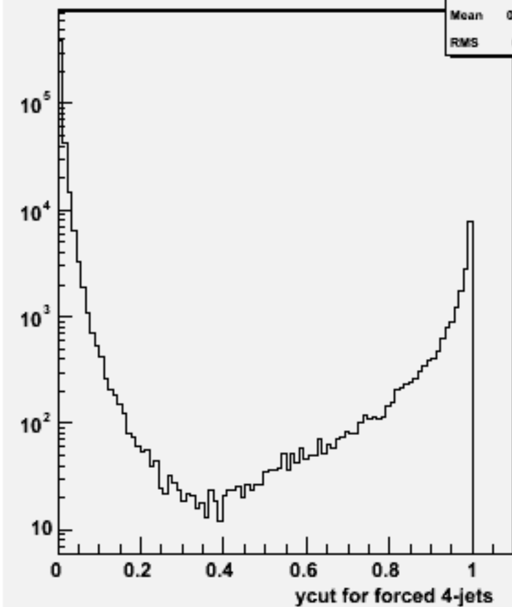
Ycut for 4-jets :w100621 e1e1e3e3_o
