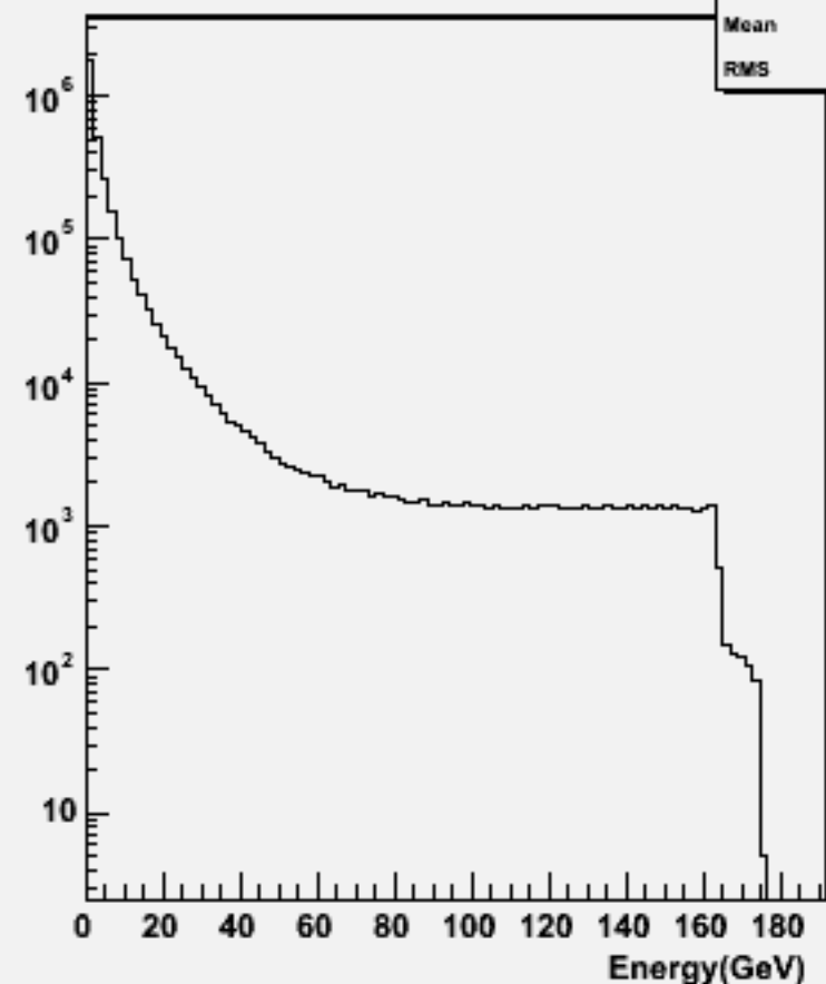
Particle Energy : w100596 cce2e2_o
