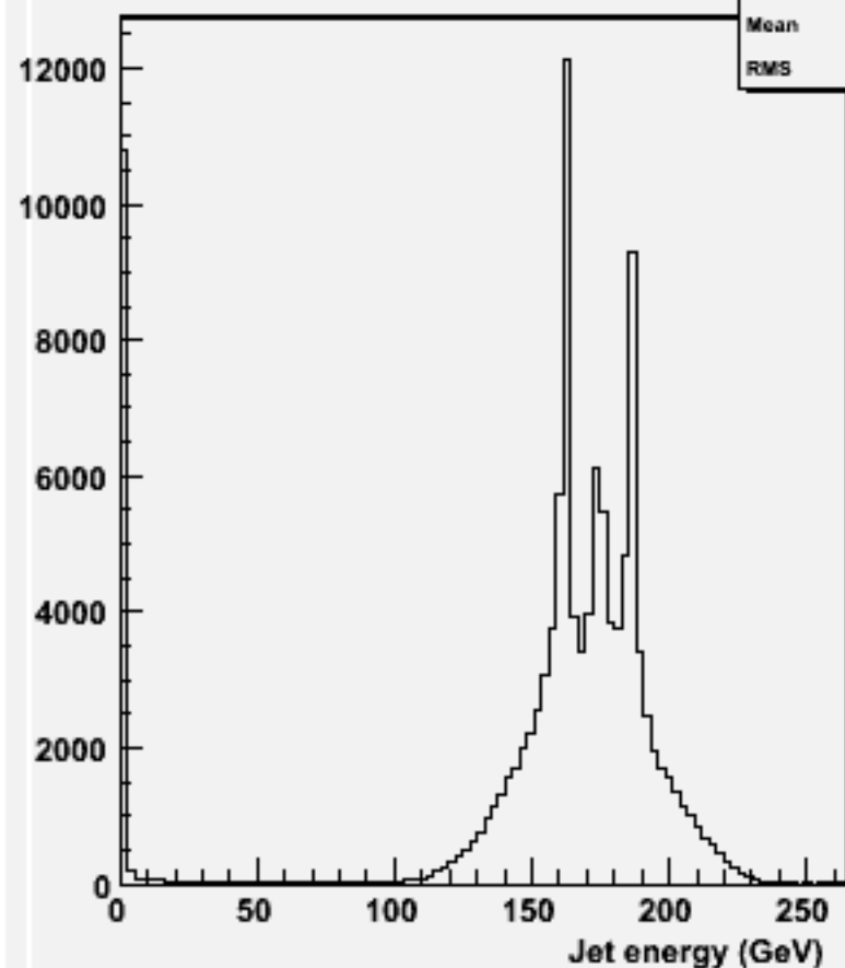
energy for 2-jets :w100596 cce2e2_o
