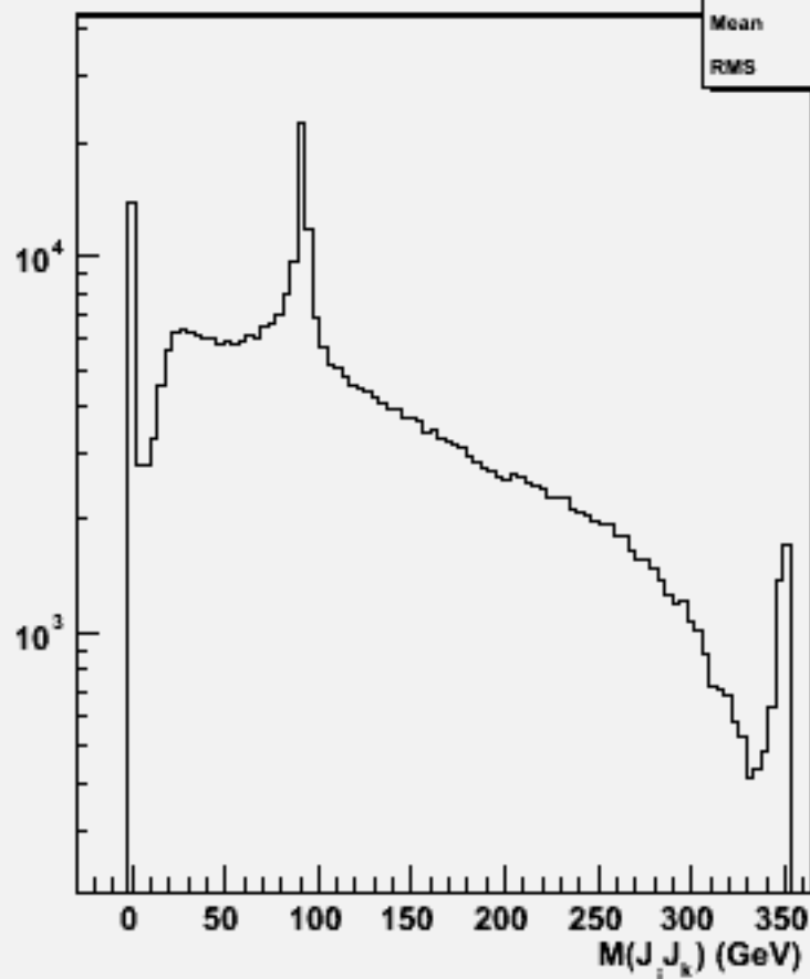
2jets mass(All comb)w100596 cce2e2_o
