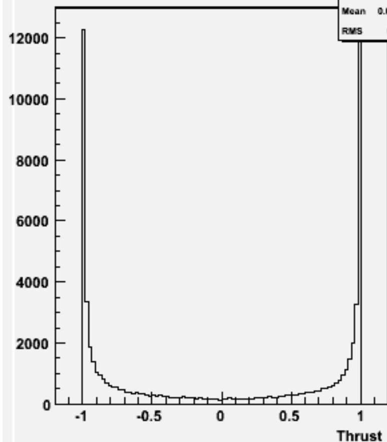
cos \Theta (thrust) w100596 cce2e2_o
