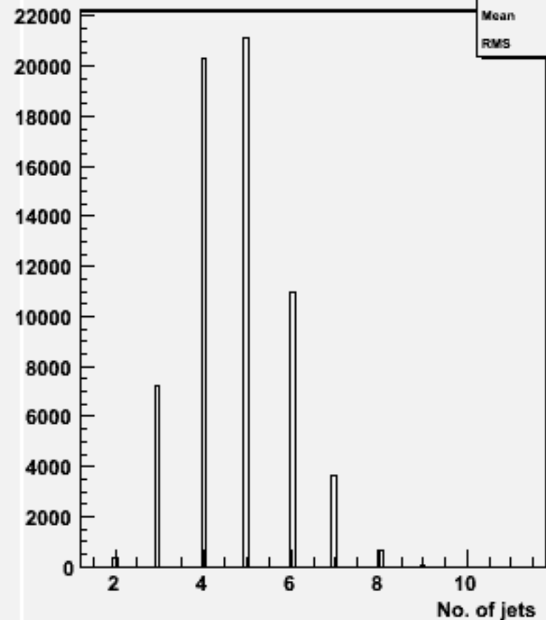
No. jets (ycut=0.001) : w100596 cce2e2_o
