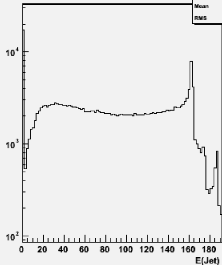
Jet energies(All jets)w100596 cce2e2_o
