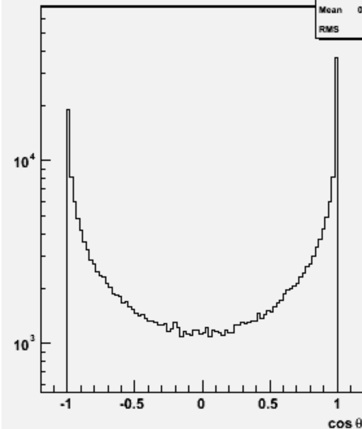
Jet cos \theta (All jets)w100596 cce2e2_o
