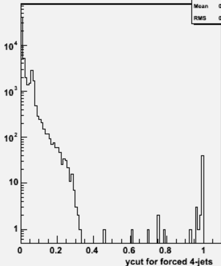
Ycut for 4-jets :w100596 cce2e2_o
