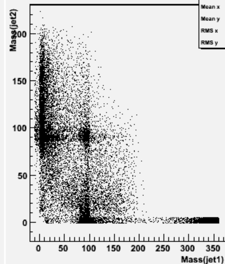
Jet mass for forced 2-jets : w100596 cce2e2_o
