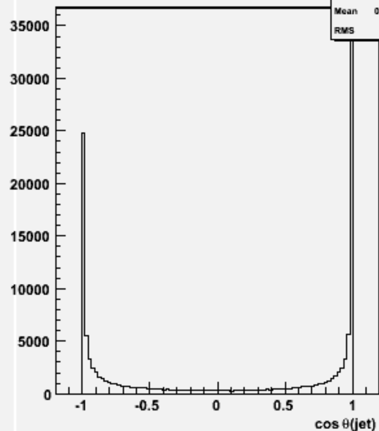
cos \theta for 2-jets :w100596 cce2e2_o
