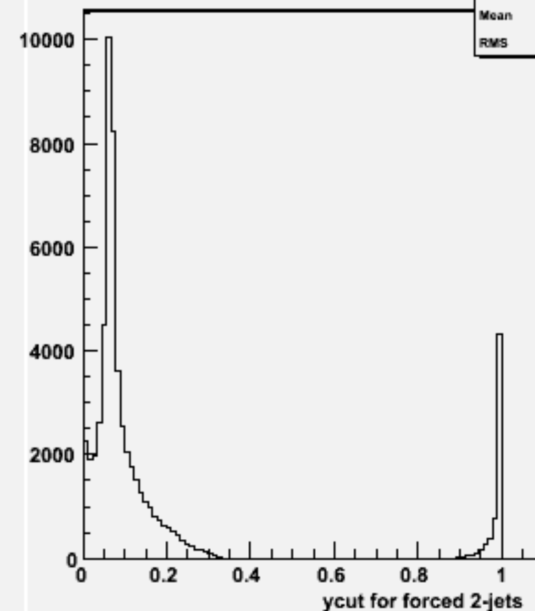
Ycut for 2-jets :w100596 cce2e2_o
