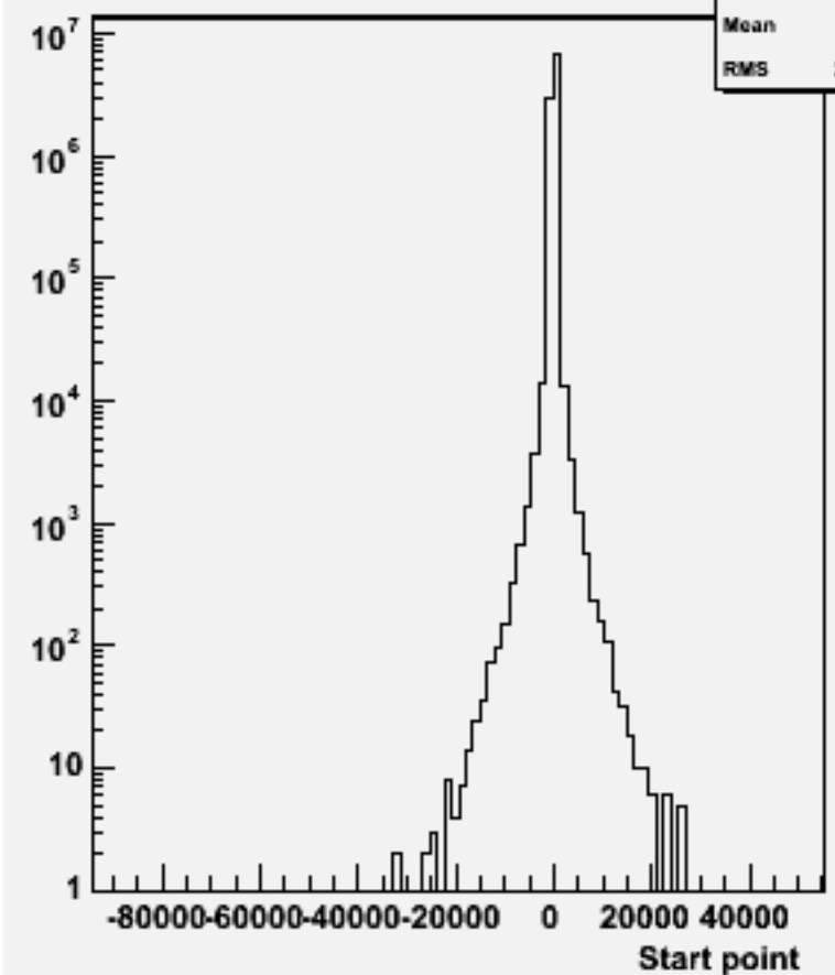
Start point Z : w100594 cce1e1_o
