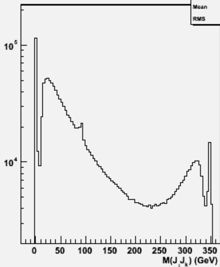
2jets mass(All comb)w100594 cce1e1_o
