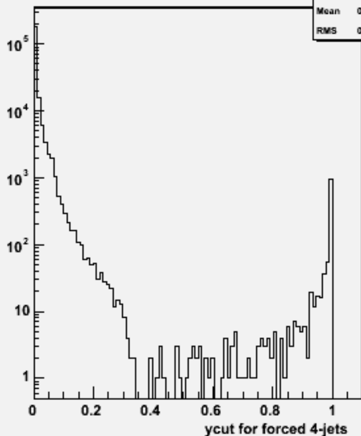
Ycut for 4-jets :w100594 cce1e1_o
