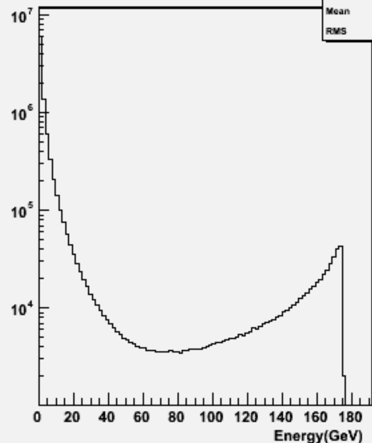
Particle Energy : w100594 cce1e1_o
