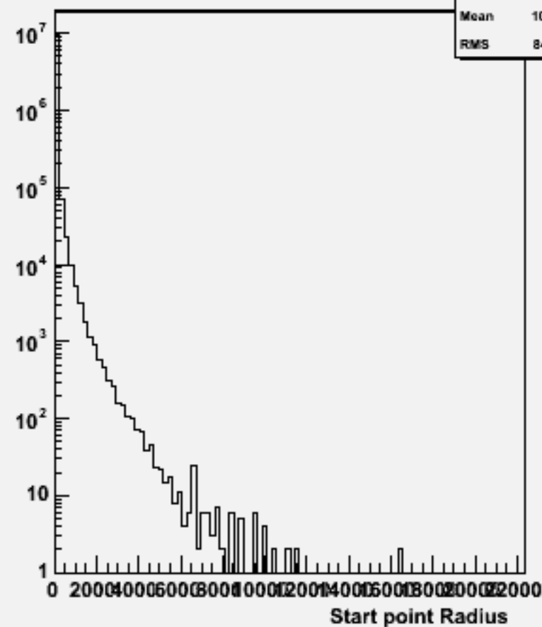
Start point R : w100594 cce1e1_o
