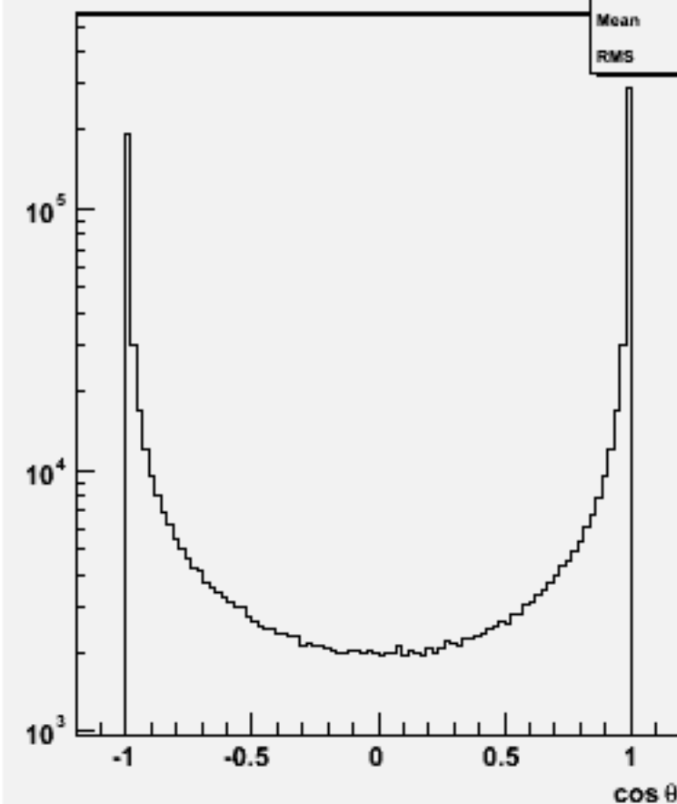
Jet cos \theta (All jets)w100594 cce1e1_o
