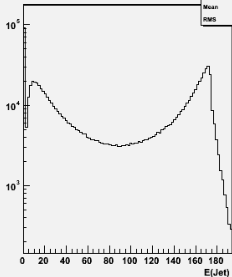
Jet energies(All jets)w100594 cce1e1_o
