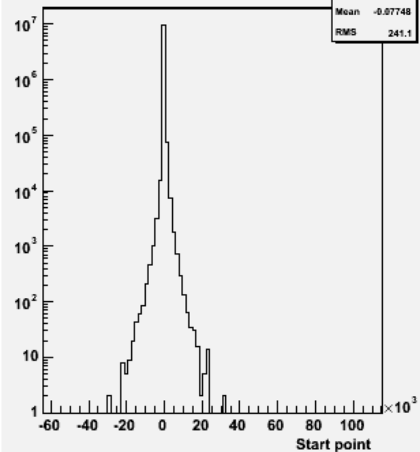
Start point Z : w100593 cce1e1_o
