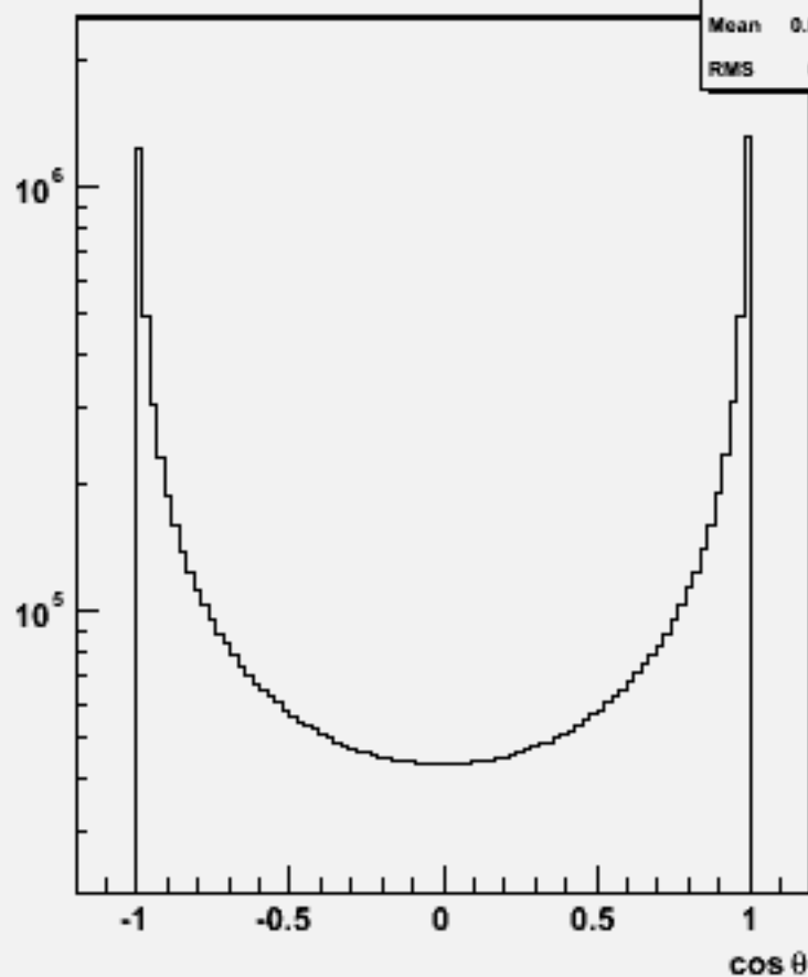
Particle cos \theta : w100593 cce1e1_o
