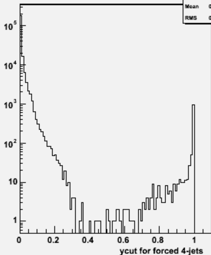
Ycut for 4-jets :w100593 cce1e1_o
