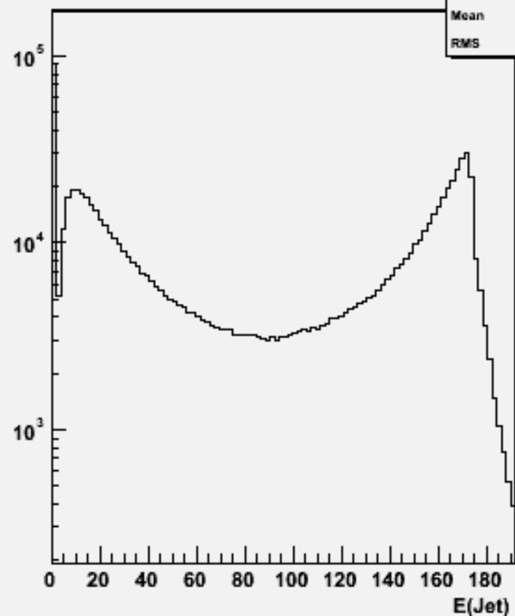
Jet energies(All jets)w100593 cce1e1_o
