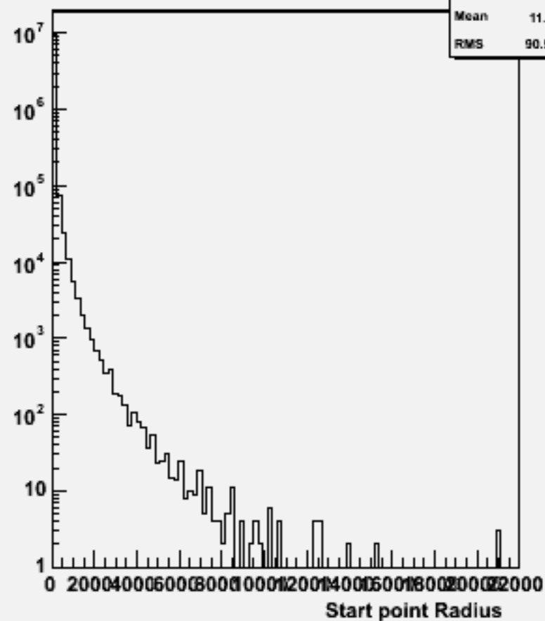
Start point R : w100593 cce1e1_o
