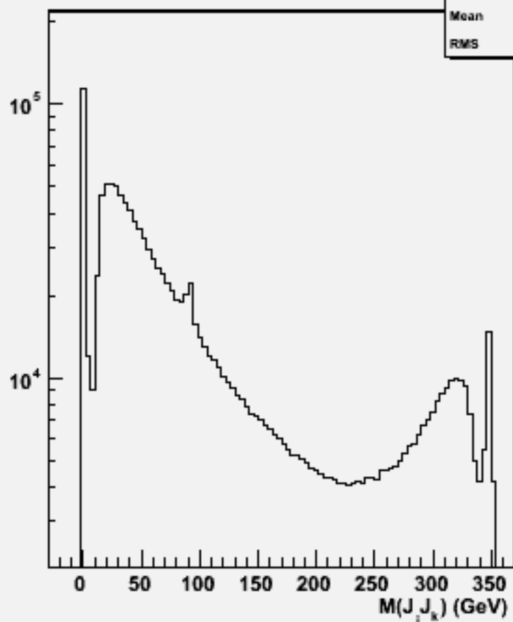
2jets mass(All comb)w100593 cce1e1_o
