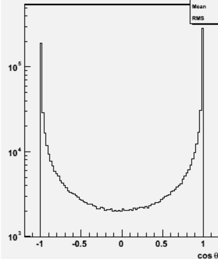
Jet cosθ (All jets)w100593 cce1e1_o
