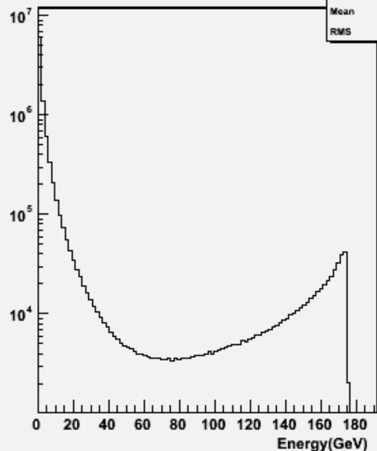
Particle Energy : w100593 cce1e1_o
